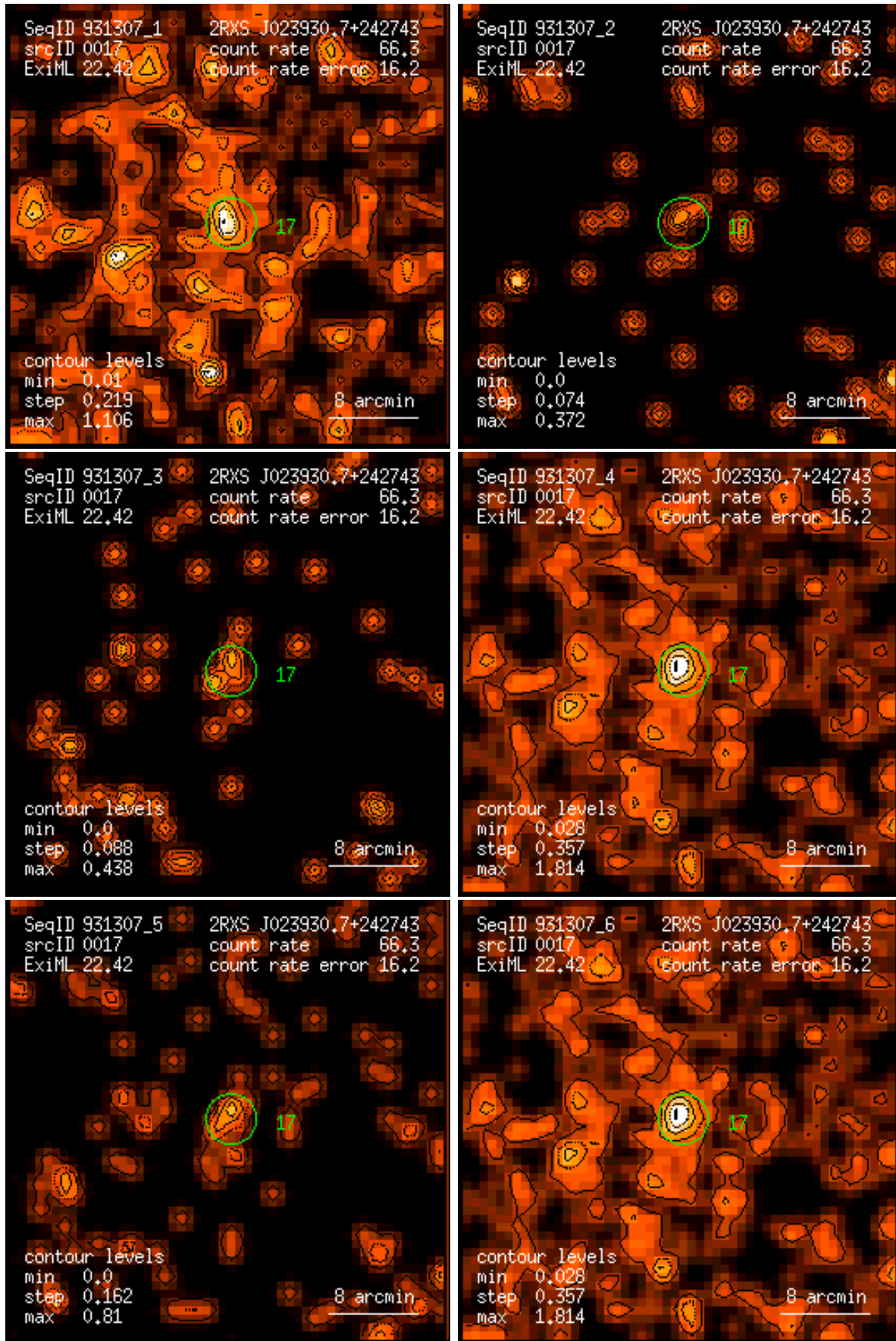
Figure 17: RASS 931307: detection 0017: band rate images, Gaussian filter: (1) PSPC channels 11 – 41, (2) 52 – 90, (3) 91 – 201, (4) 11 – 235, (5) 52 – 201, (6) 11 – 201. Broad band rates in counts/ks. Band rate contour levels in counts/ks/arcmin 2 .
