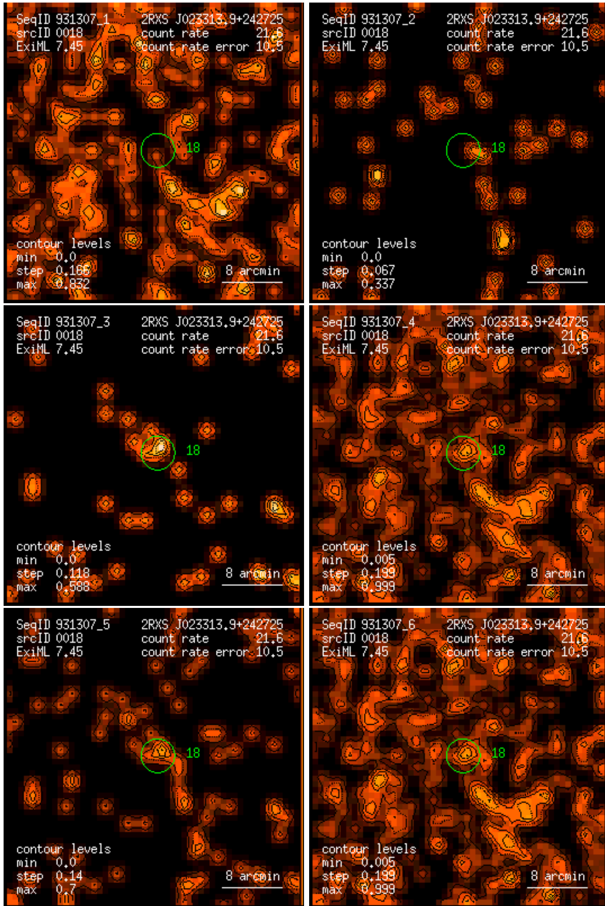
Figure 18: RASS 931307: detection 0018: band rate images, Gaussian filter: (1) PSPC channels 11 – 41, (2) 52 – 90, (3) 91 – 201, (4) 11 – 235, (5) 52 – 201, (6) 11 – 201. Broad band rates in counts/ks. Band rate contour levels in counts/ks/arcmin 2 .
