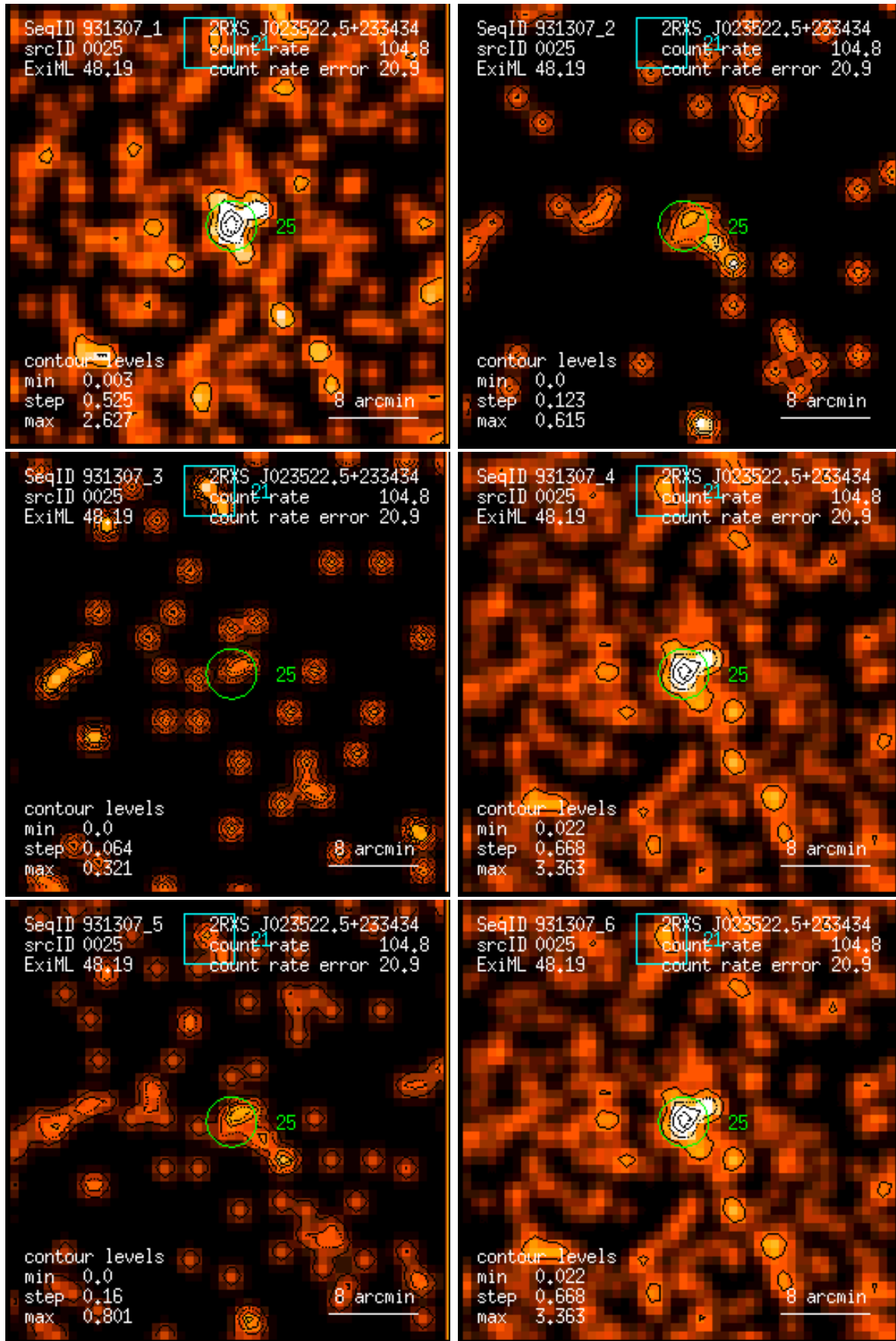
Figure 25: RASS 931307: detection 0025: band rate images, Gaussian filter: (1) PSPC channels 11 – 41, (2) 52 – 90, (3) 91 – 201, (4) 11 – 235, (5) 52 – 201, (6) 11 – 201. Broad band rates in counts/ks. Band rate contour levels in counts/ks/arcmin 2 .
