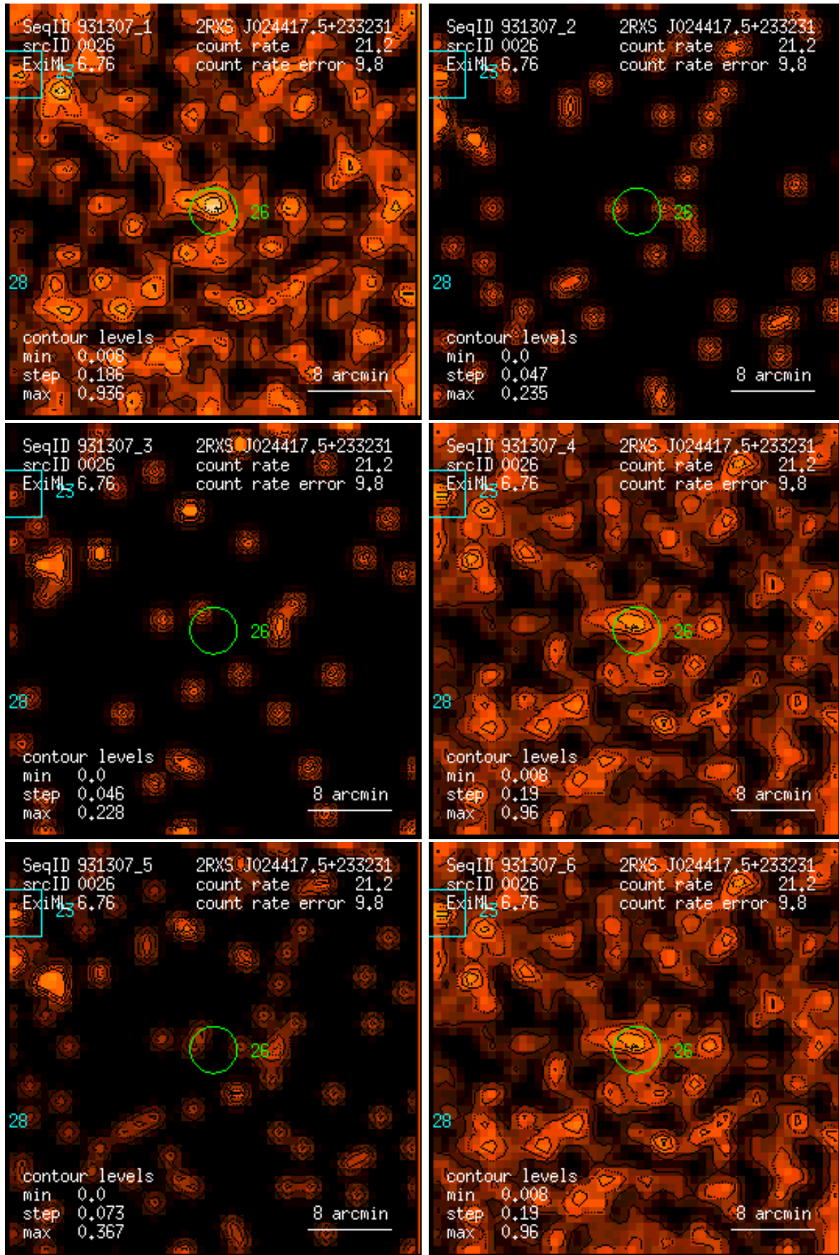
Figure 26: RASS 931307: detection 0026: band rate images, Gaussian filter: (1) PSPC channels 11 – 41, (2) 52 – 90, (3) 91 – 201, (4) 11 – 235, (5) 52 – 201, (6) 11 – 201. Broad band rates in counts/ks. Band rate contour levels in counts/ks/arcmin 2 .
