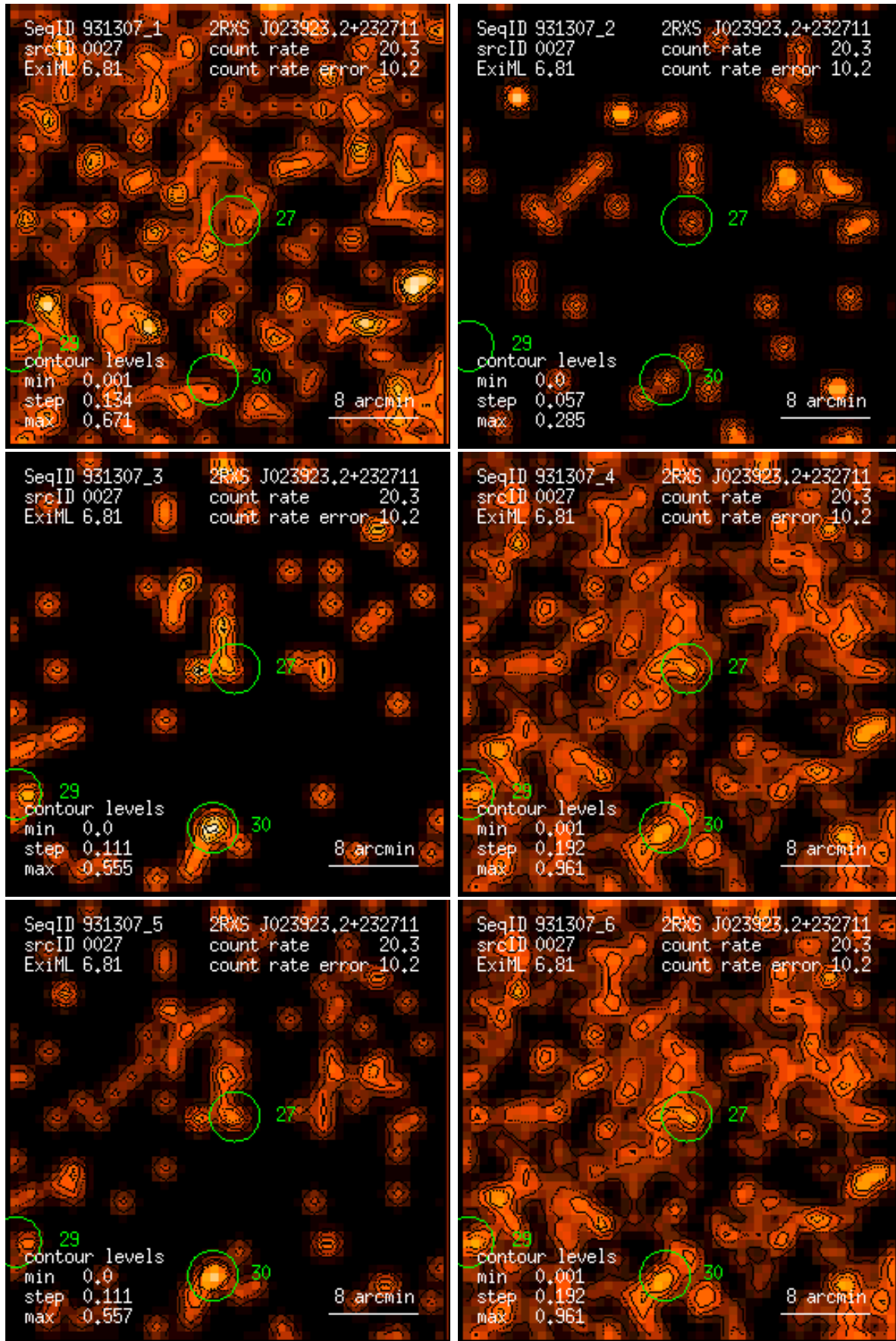
Figure 27: RASS 931307: detection 0027: band rate images, Gaussian filter: (1) PSPC channels 11 – 41, (2) 52 – 90, (3) 91 – 201, (4) 11 – 235, (5) 52 – 201, (6) 11 – 201. Broad band rates in counts/ks. Band rate contour levels in counts/ks/arcmin 2 .
