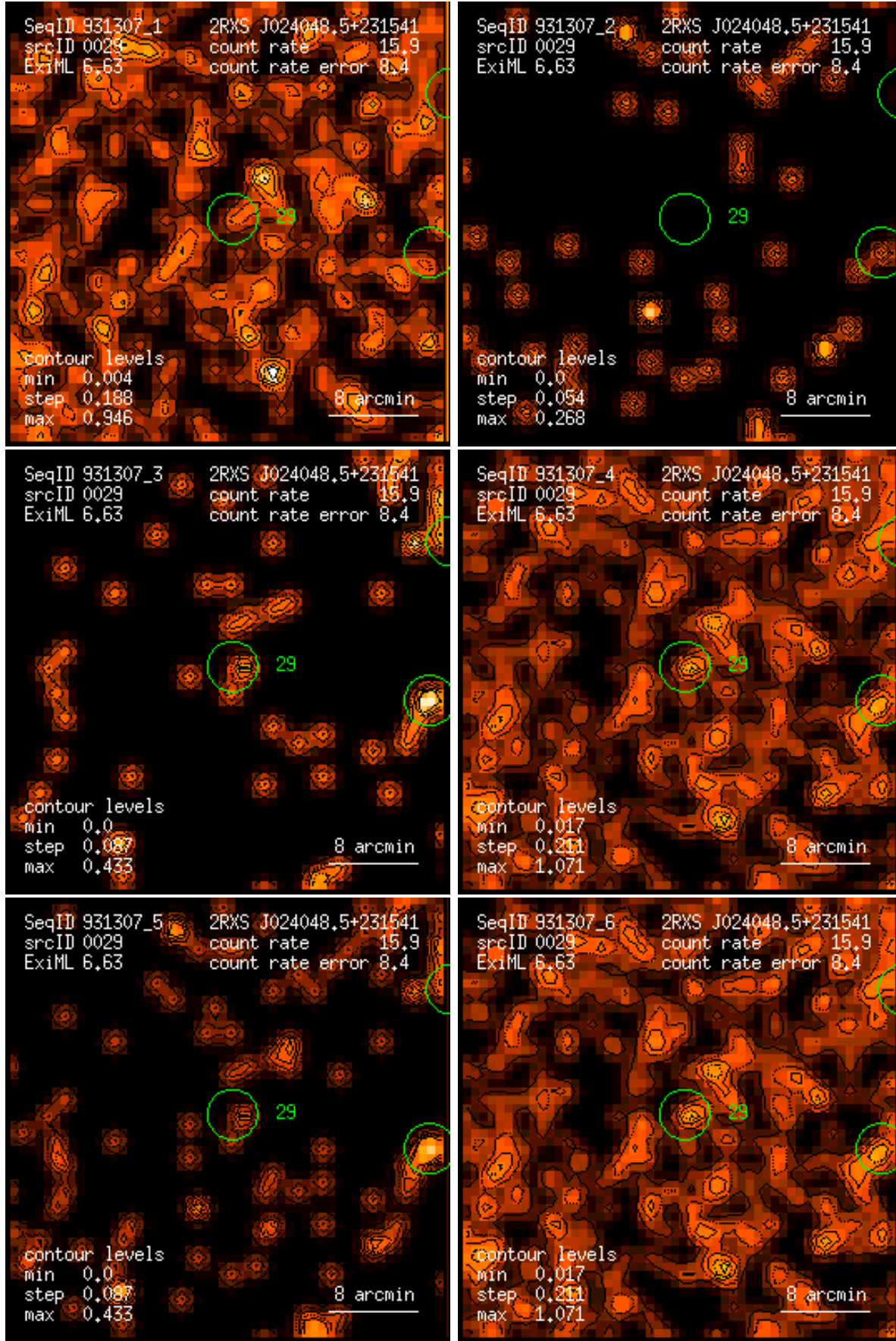
Figure 29: RASS 931307: detection 0029: band rate images, Gaussian filter: (1) PSPC channels 11 – 41, (2) 52 – 90, (3) 91 – 201, (4) 11 – 235, (5) 52 – 201, (6) 11 – 201. Broad band rates in counts/ks. Band rate contour levels in counts/ks/arcmin 2 .
