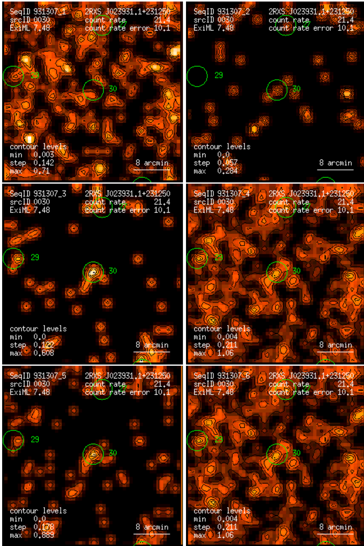
Figure 30: RASS 931307: detection 0030: band rate images, Gaussian filter: (1) PSPC channels 11 – 41, (2) 52 – 90, (3) 91 – 201, (4) 11 – 235, (5) 52 – 201, (6) 11 – 201. Broad band rates in counts/ks. Band rate contour levels in counts/ks/arcmin 2 .
