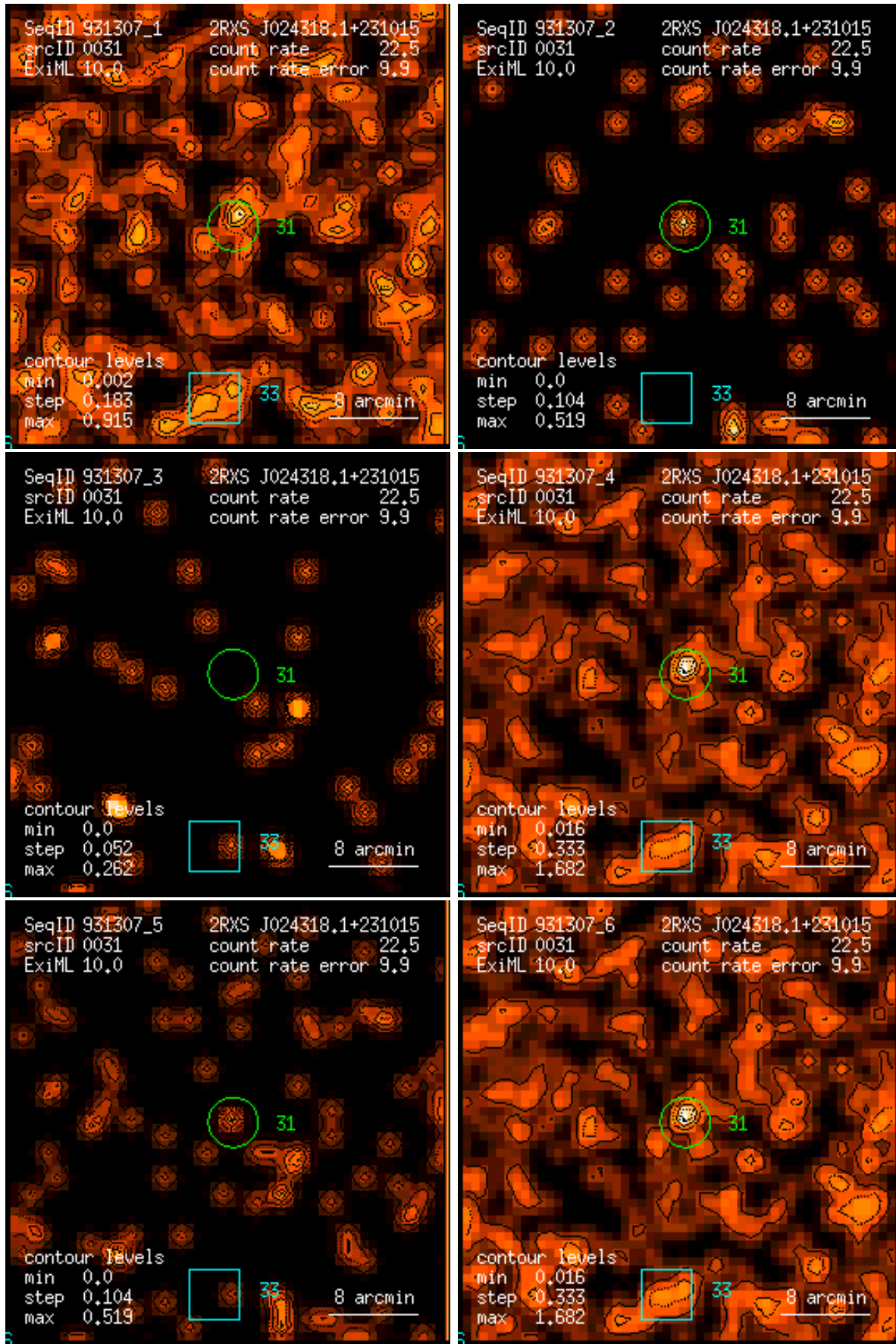
Figure 31: RASS 931307: detection 0031: band rate images, Gaussian filter: (1) PSPC channels 11 – 41, (2) 52 – 90, (3) 91 – 201, (4) 11 – 235, (5) 52 – 201, (6) 11 – 201. Broad band rates in counts/ks. Band rate contour levels in counts/ks/arcmin 2 .
