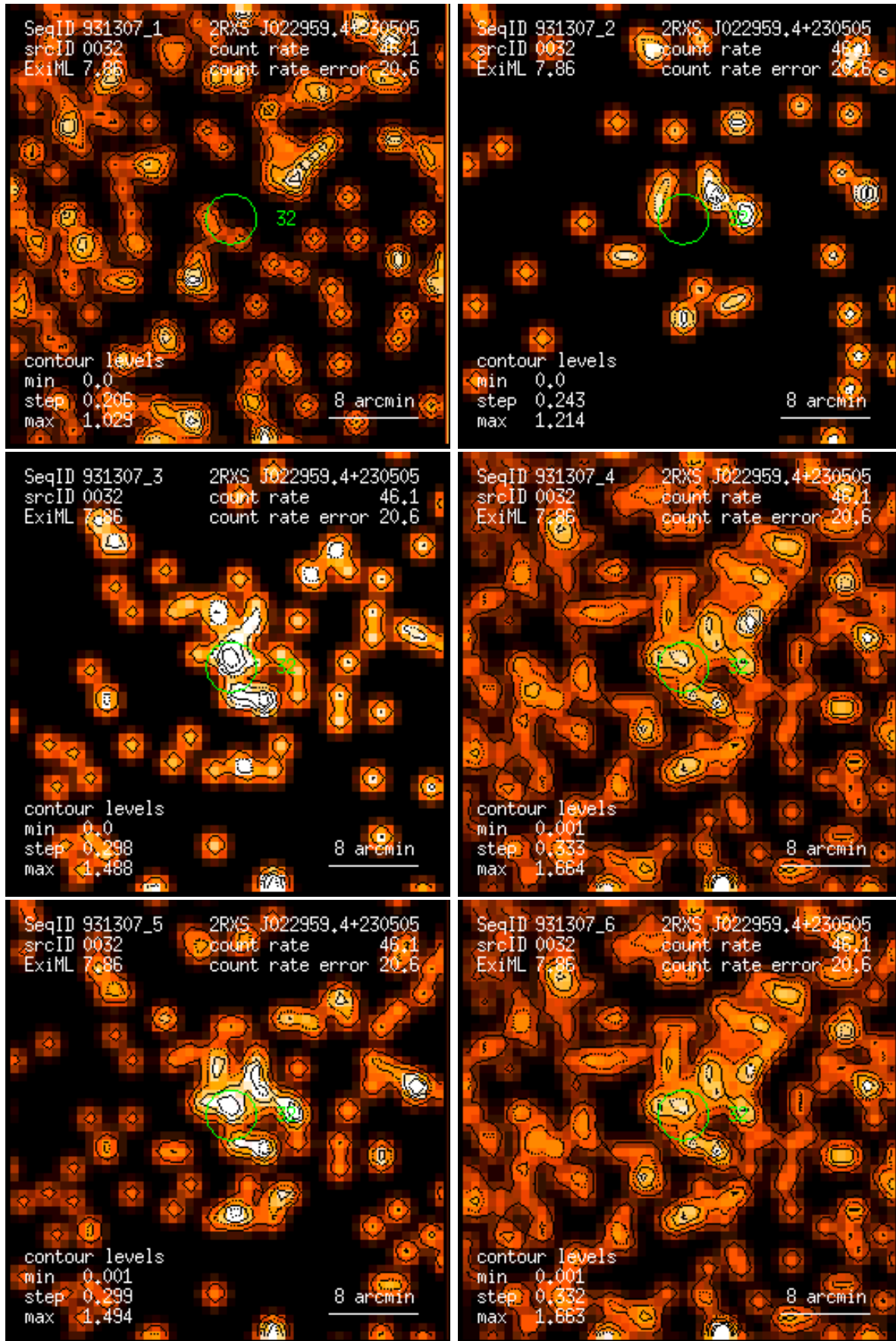
Figure 32: RASS 931307: detection 0032: band rate images, Gaussian filter: (1) PSPC channels 11 – 41, (2) 52 – 90, (3) 91 – 201, (4) 11 – 235, (5) 52 – 201, (6) 11 – 201. Broad band rates in counts/ks. Band rate contour levels in counts/ks/arcmin 2 .
