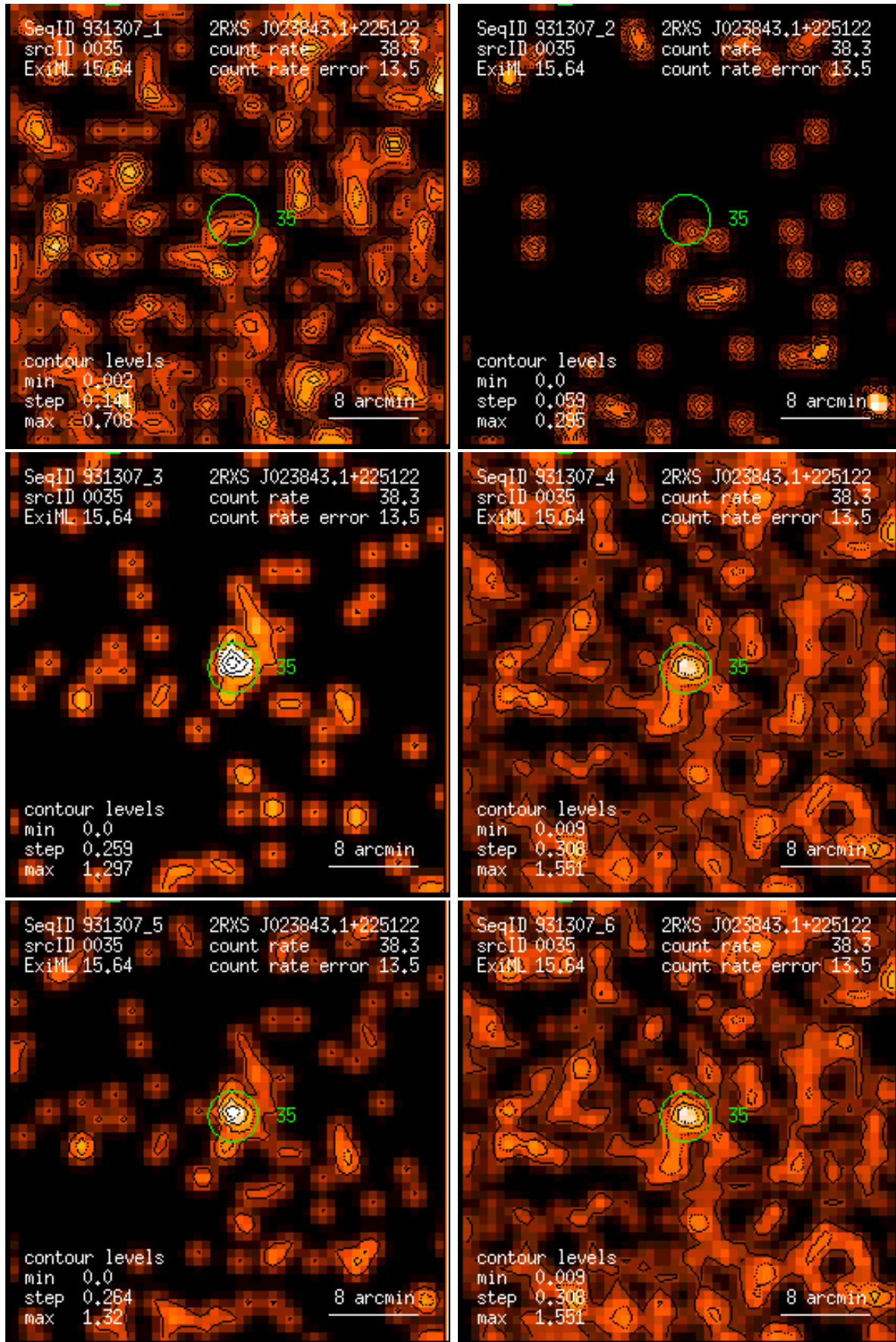
Figure 35: RASS 931307: detection 0035: band rate images, Gaussian filter: (1) PSPC channels 11 – 41, (2) 52 – 90, (3) 91 – 201, (4) 11 – 235, (5) 52 – 201, (6) 11 – 201. Broad band rates in counts/ks. Band rate contour levels in counts/ks/arcmin 2 .
