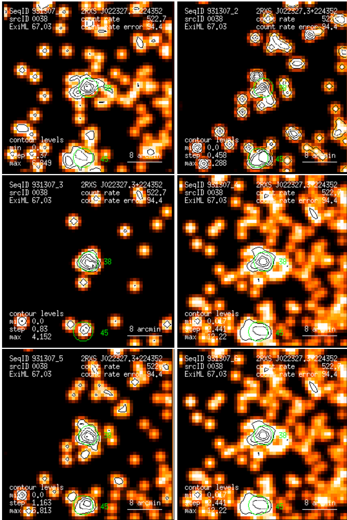
Figure 38: RASS 931307: detection 0038: band rate images, Gaussian filter: (1) PSPC channels 11 – 41, (2) 52 – 90, (3) 91 – 201, (4) 11 – 235, (5) 52 – 201, (6) 11 – 201. Broad band rates in counts/ks. Band rate contour levels in counts/ks/arcmin 2 .
