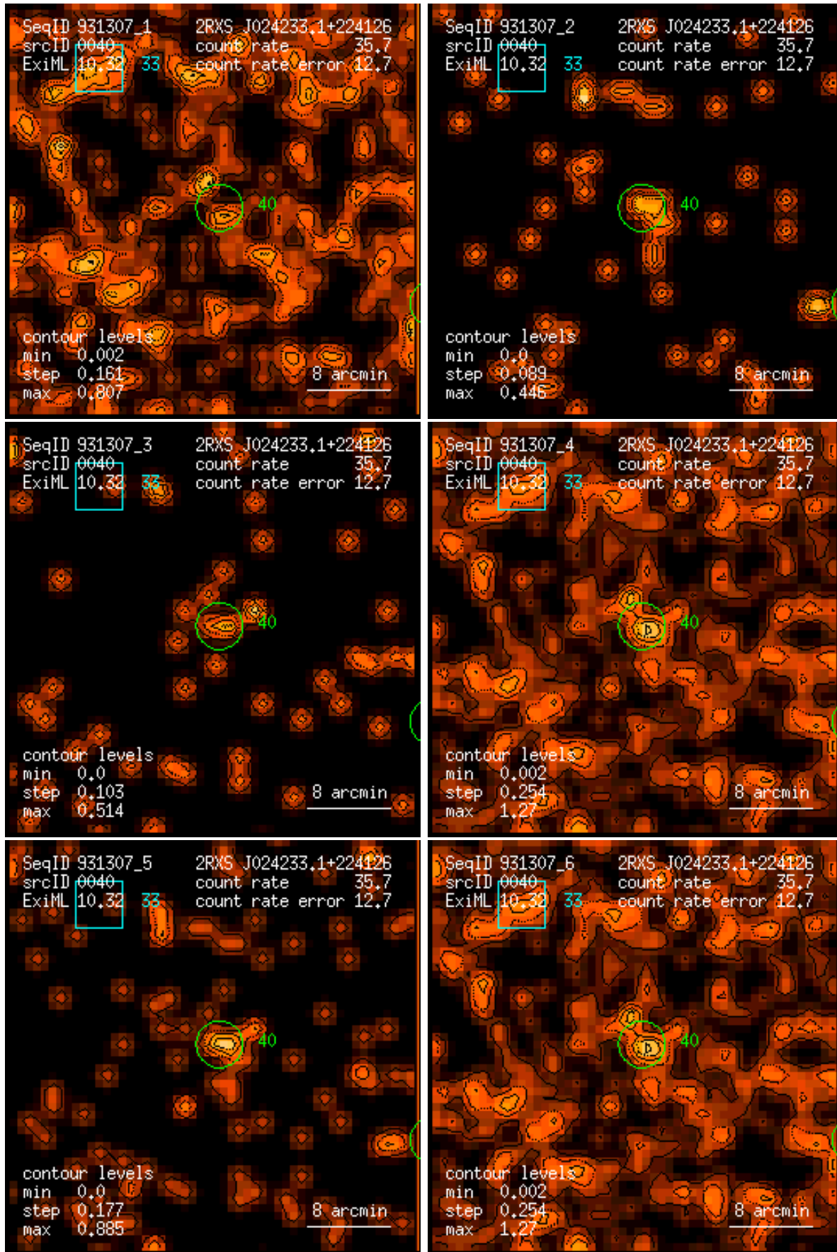
Figure 40: RASS 931307: detection 0040: band rate images, Gaussian filter: (1) PSPC channels 11 – 41, (2) 52 – 90, (3) 91 – 201, (4) 11 – 235, (5) 52 – 201, (6) 11 – 201. Broad band rates in counts/ks. Band rate contour levels in counts/ks/arcmin 2 .
