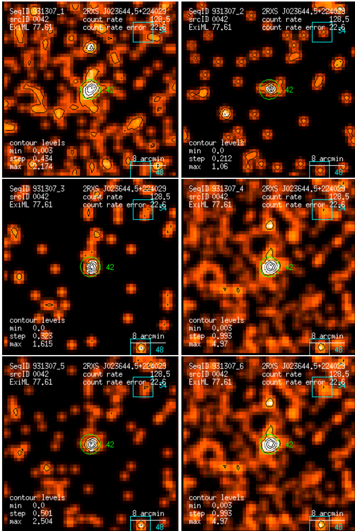
Figure 42: RASS 931307: detection 0042: band rate images, Gaussian filter: (1) PSPC channels 11 – 41, (2) 52 – 90, (3) 91 – 201, (4) 11 – 235, (5) 52 – 201, (6) 11 – 201. Broad band rates in counts/ks. Band rate contour levels in counts/ks/arcmin 2 .
