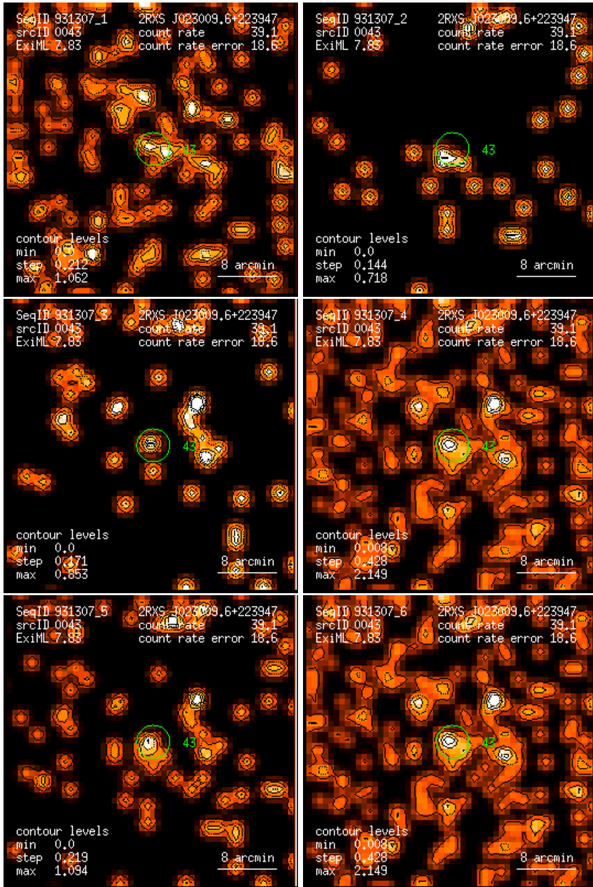
Figure 43: RASS 931307: detection 0043: band rate images, Gaussian filter: (1) PSPC channels 11 – 41, (2) 52 – 90, (3) 91 – 201, (4) 11 – 235, (5) 52 – 201, (6) 11 – 201. Broad band rates in counts/ks. Band rate contour levels in counts/ks/arcmin 2 .
