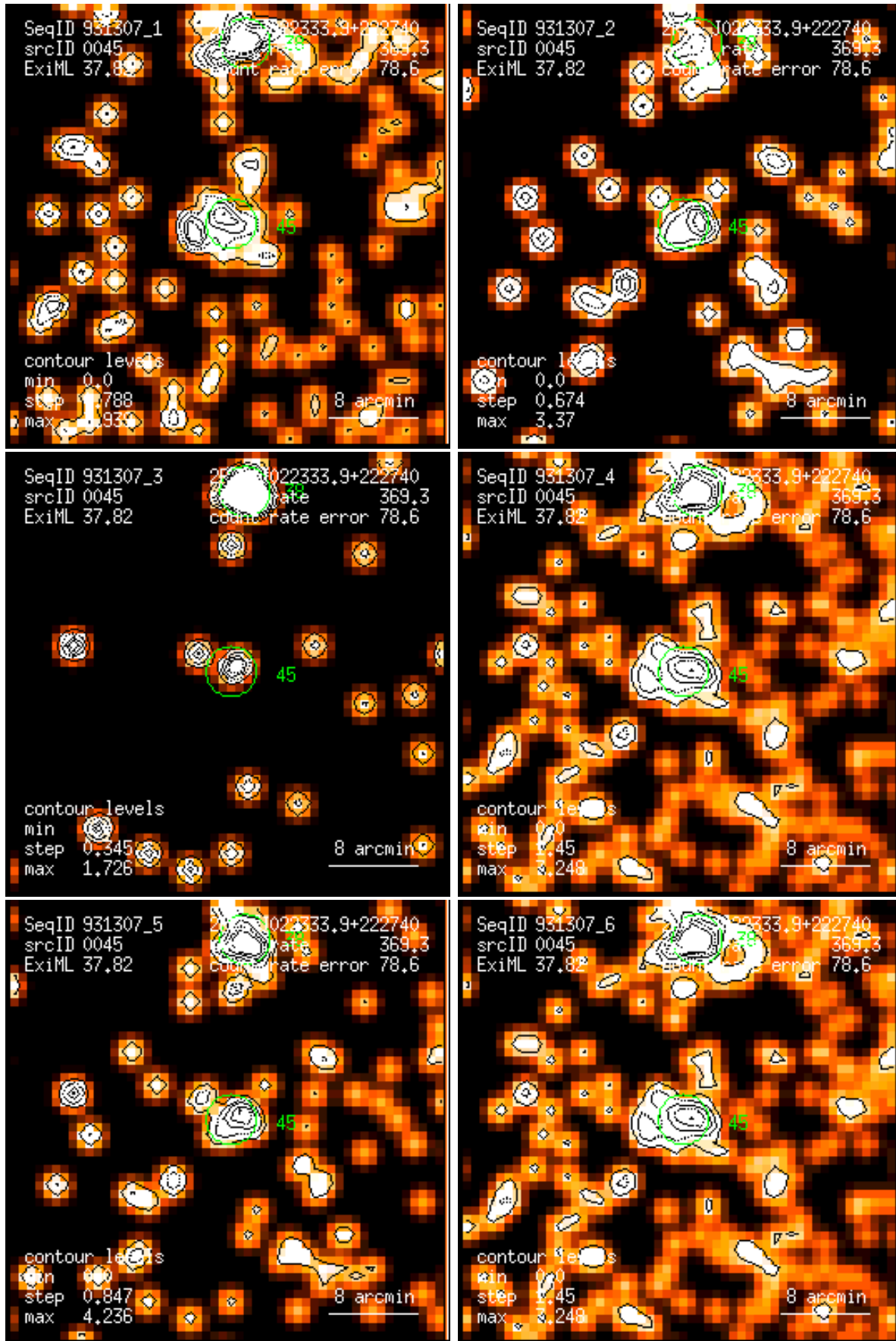
Figure 45: RASS 931307: detection 0045: band rate images, Gaussian filter: (1) PSPC channels 11 – 41, (2) 52 – 90, (3) 91 – 201, (4) 11 – 235, (5) 52 – 201, (6) 11 – 201. Broad band rates in counts/ks. Band rate contour levels in counts/ks/arcmin 2 .
