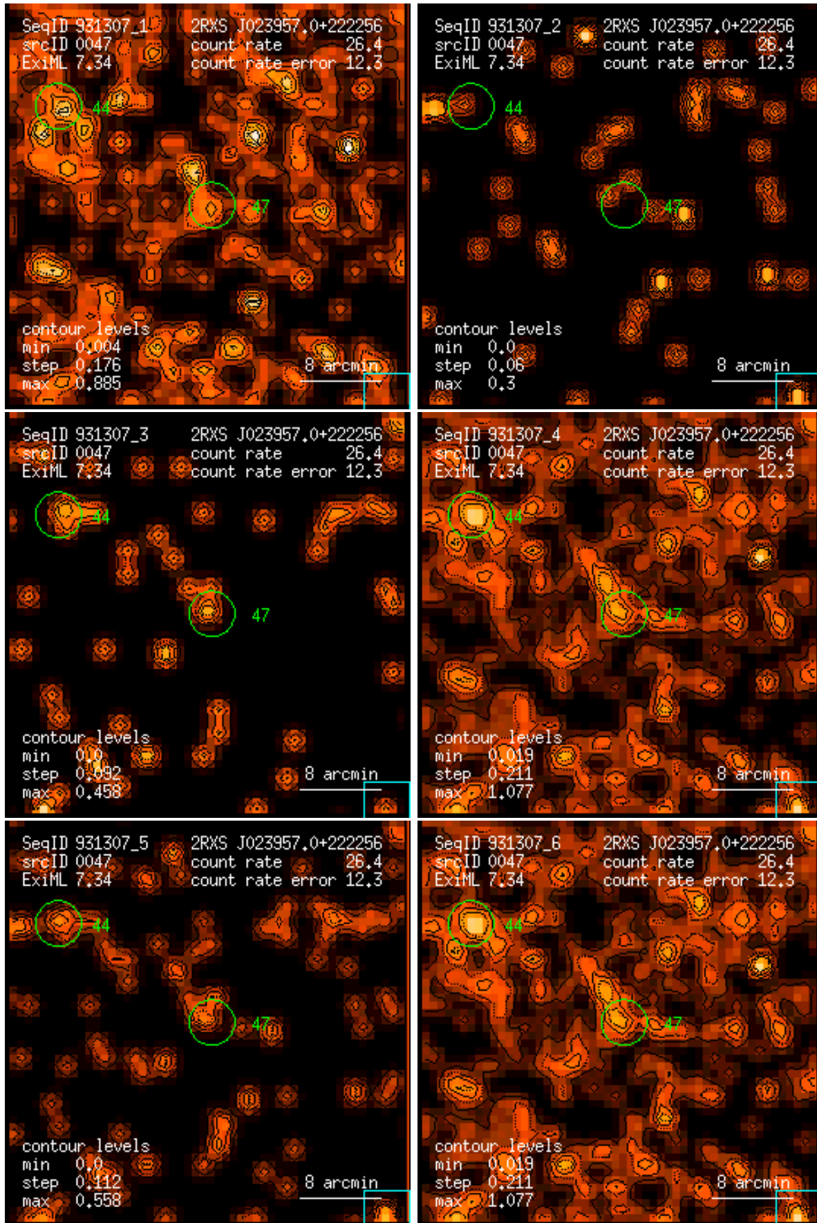
Figure 47: RASS 931307: detection 0047: band rate images, Gaussian filter: (1) PSPC channels 11 – 41, (2) 52 – 90, (3) 91 – 201, (4) 11 – 235, (5) 52 – 201, (6) 11 – 201. Broad band rates in counts/ks. Band rate contour levels in counts/ks/arcmin 2 .
