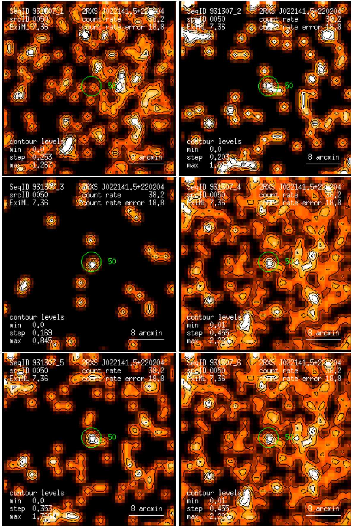
Figure 50: RASS 931307: detection 0050: band rate images, Gaussian filter: (1) PSPC channels 11 – 41, (2) 52 – 90, (3) 91 – 201, (4) 11 – 235, (5) 52 – 201, (6) 11 – 201. Broad band rates in counts/ks. Band rate contour levels in counts/ks/arcmin 2 .
