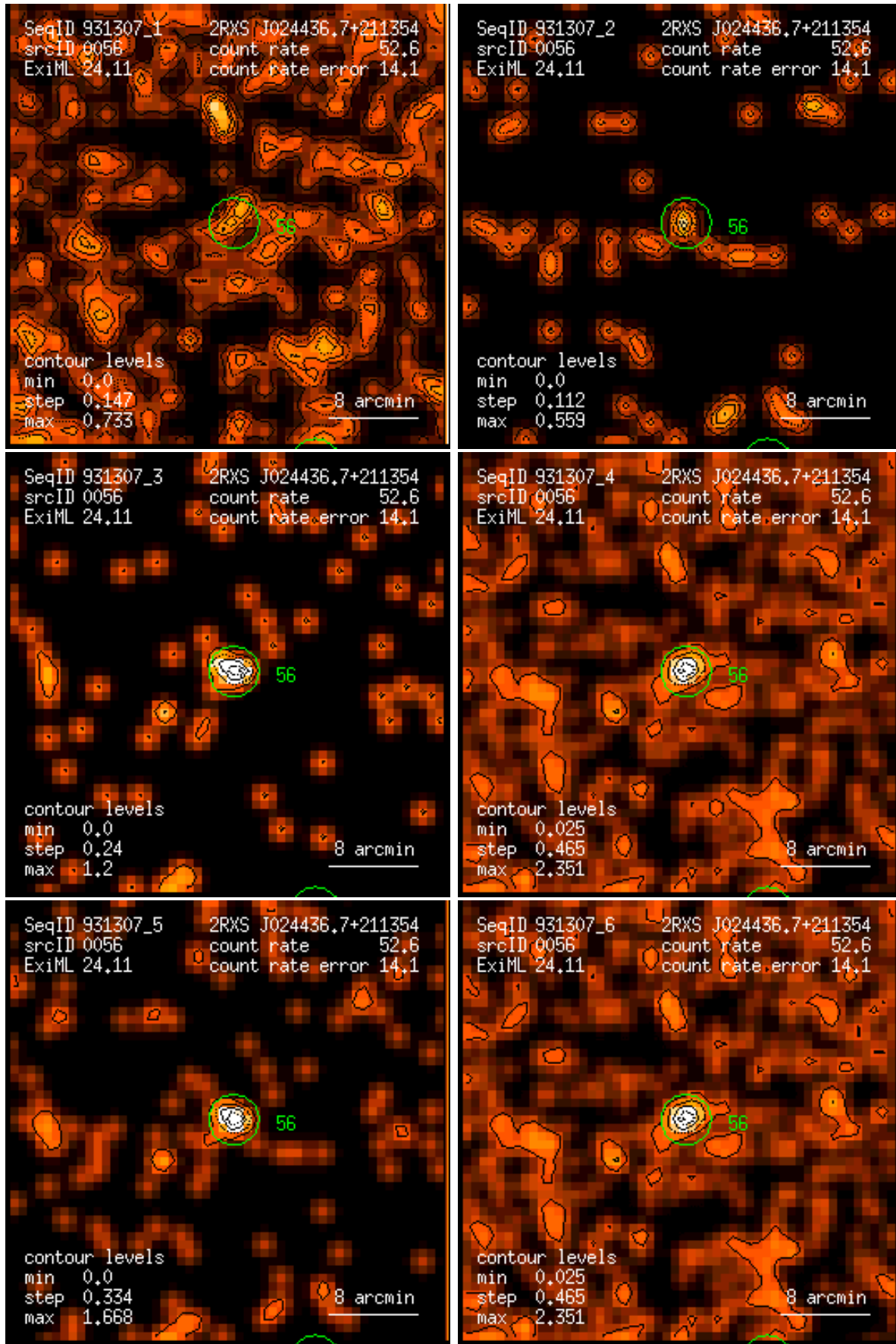
Figure 56: RASS 931307: detection 0056: band rate images, Gaussian filter: (1) PSPC channels 11 – 41, (2) 52 – 90, (3) 91 – 201, (4) 11 – 235, (5) 52 – 201, (6) 11 – 201. Broad band rates in counts/ks. Band rate contour levels in counts/ks/arcmin 2 .
