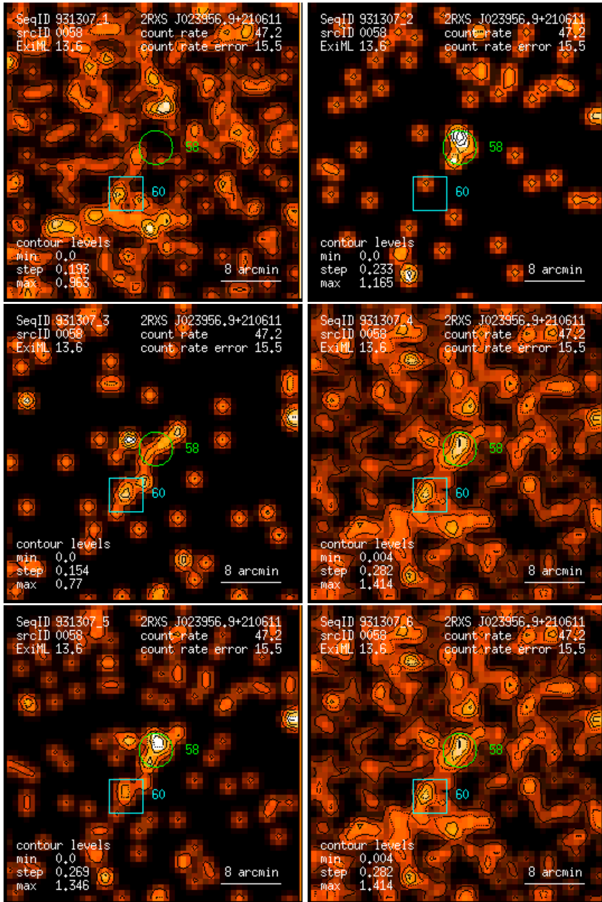
Figure 58: RASS 931307: detection 0058: band rate images, Gaussian filter: (1) PSPC channels 11 – 41, (2) 52 – 90, (3) 91 – 201, (4) 11 – 235, (5) 52 – 201, (6) 11 – 201. Broad band rates in counts/ks. Band rate contour levels in counts/ks/arcmin 2 .
