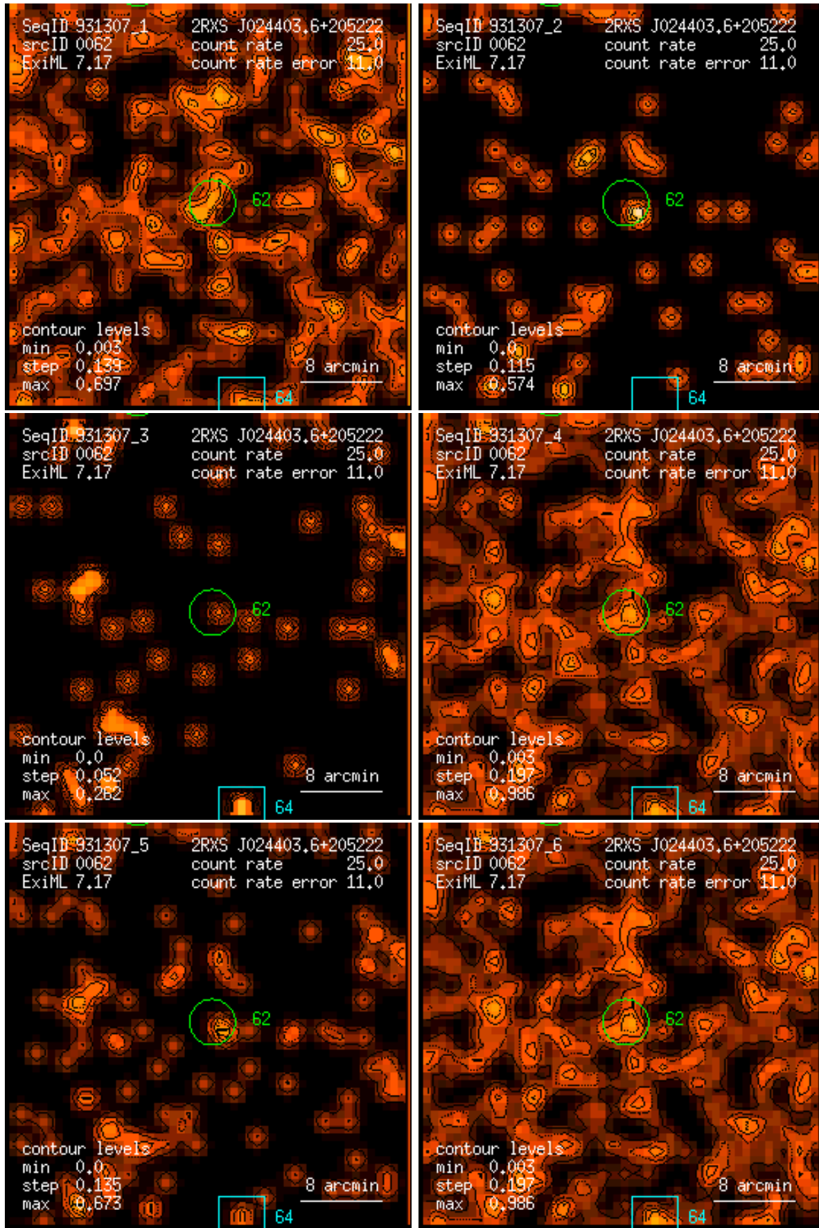
Figure 62: RASS 931307: detection 0062: band rate images, Gaussian filter: (1) PSPC channels 11 – 41, (2) 52 – 90, (3) 91 – 201, (4) 11 – 235, (5) 52 – 201, (6) 11 – 201. Broad band rates in counts/ks. Band rate contour levels in counts/ks/arcmin 2 .
