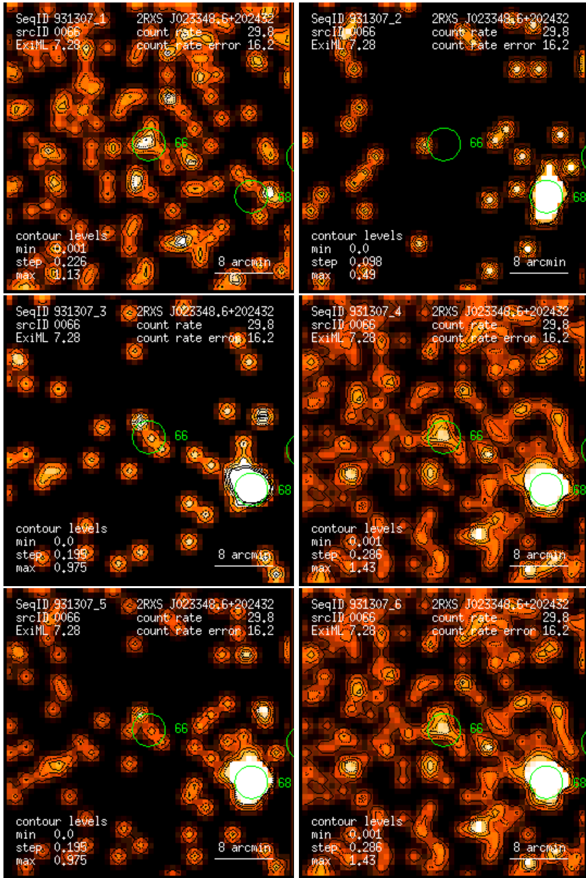
Figure 66: RASS 931307: detection 0066: band rate images, Gaussian filter: (1) PSPC channels 11 – 41, (2) 52 – 90, (3) 91 – 201, (4) 11 – 235, (5) 52 – 201, (6) 11 – 201. Broad band rates in counts/ks. Band rate contour levels in counts/ks/arcmin 2 .
