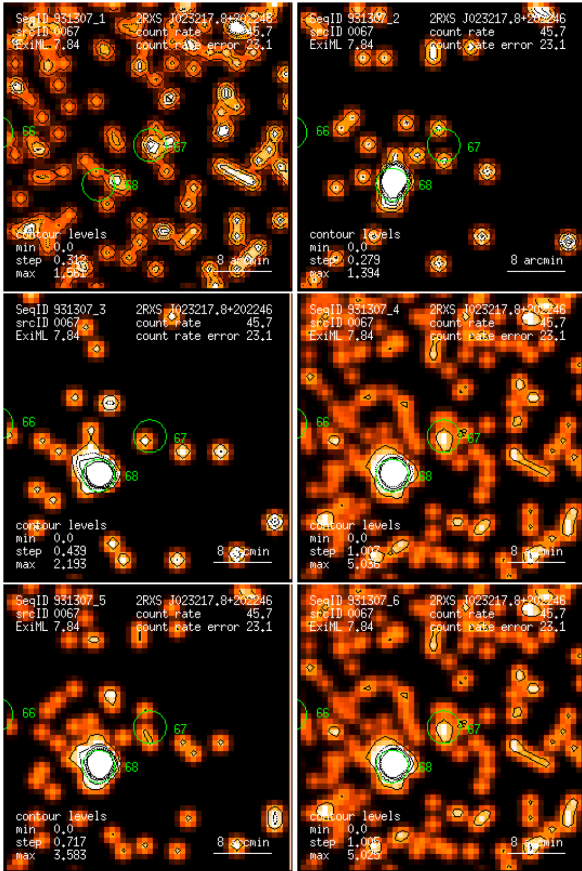
Figure 67: RASS 931307: detection 0067: band rate images, Gaussian filter: (1) PSPC channels 11 – 41, (2) 52 – 90, (3) 91 – 201, (4) 11 – 235, (5) 52 – 201, (6) 11 – 201. Broad band rates in counts/ks. Band rate contour levels in counts/ks/arcmin 2 .
