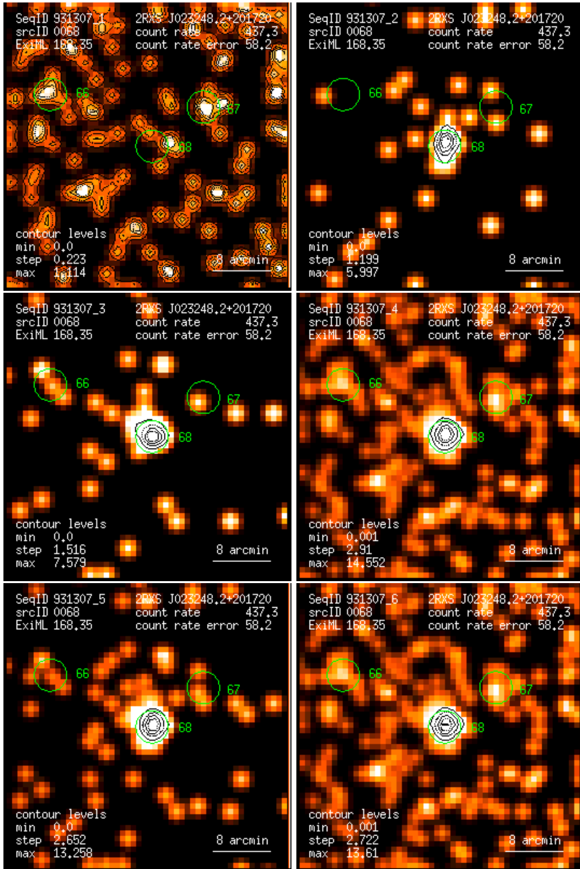
Figure 68: RASS 931307: detection 0068: band rate images, Gaussian filter: (1) PSPC channels 11 – 41, (2) 52 – 90, (3) 91 – 201, (4) 11 – 235, (5) 52 – 201, (6) 11 – 201. Broad band rates in counts/ks. Band rate contour levels in counts/ks/arcmin 2 .
