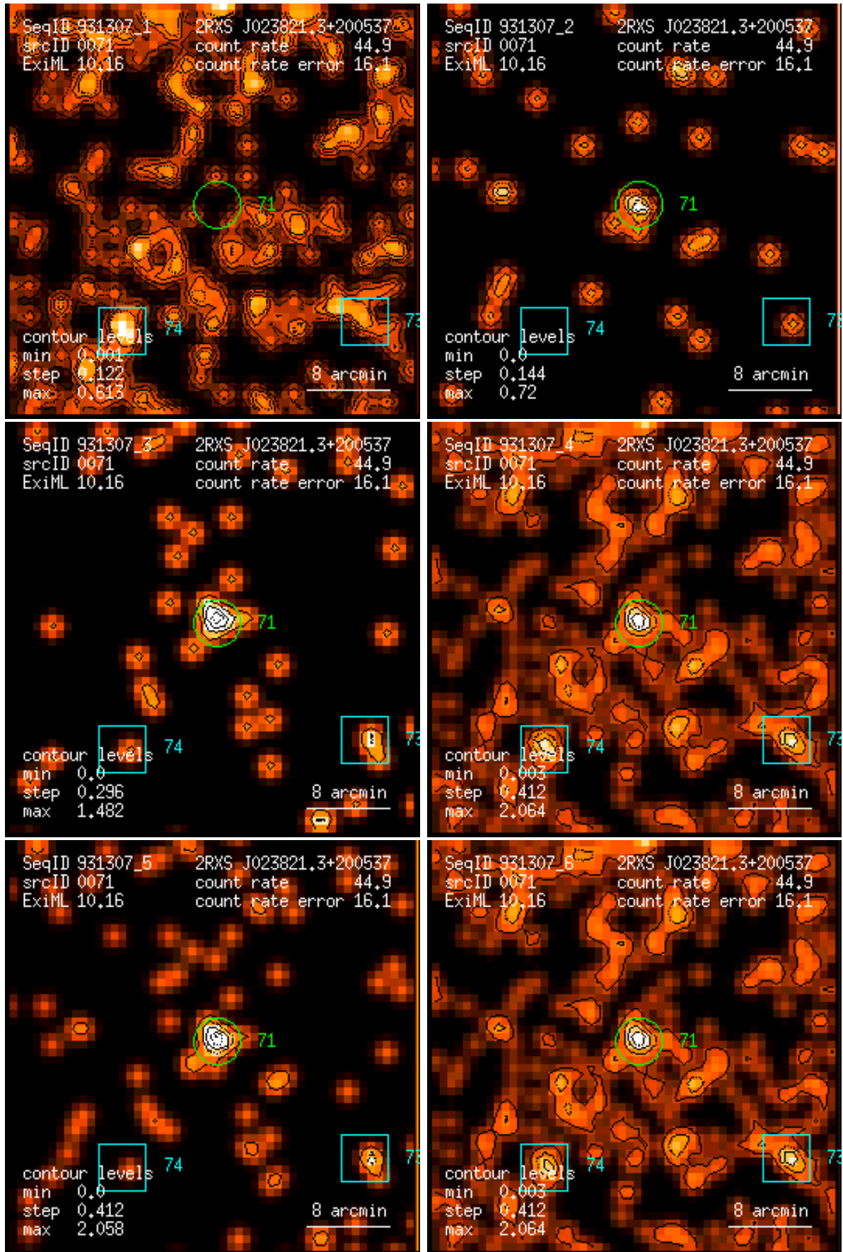
Figure 71: RASS 931307: detection 0071: band rate images, Gaussian filter: (1) PSPC channels 11 – 41, (2) 52 – 90, (3) 91 – 201, (4) 11 – 235, (5) 52 – 201, (6) 11 – 201. Broad band rates in counts/ks. Band rate contour levels in counts/ks/arcmin 2 .
