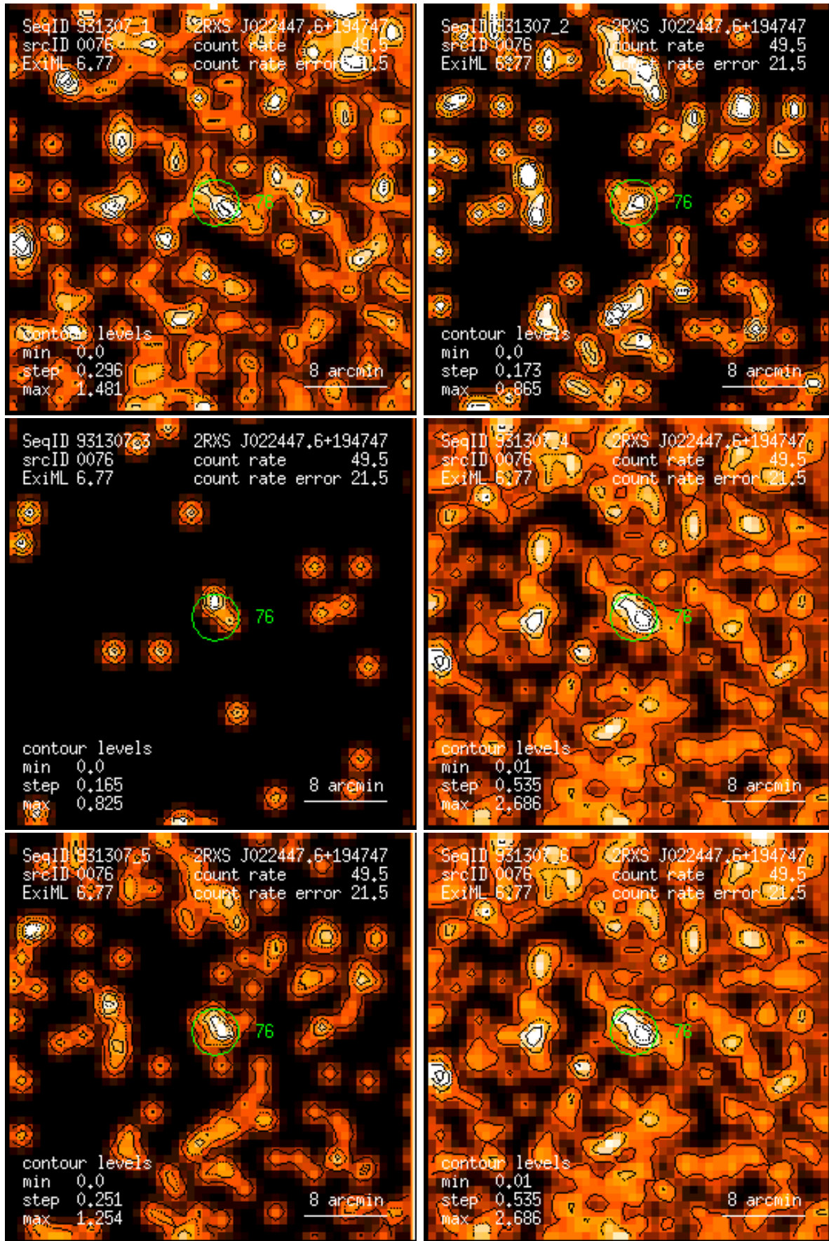
Figure 76: RASS 931307: detection 0076: band rate images, Gaussian filter: (1) PSPC channels 11 – 41, (2) 52 – 90, (3) 91 – 201, (4) 11 – 235, (5) 52 – 201, (6) 11 – 201. Broad band rates in counts/ks. Band rate contour levels in counts/ks/arcmin 2 .
