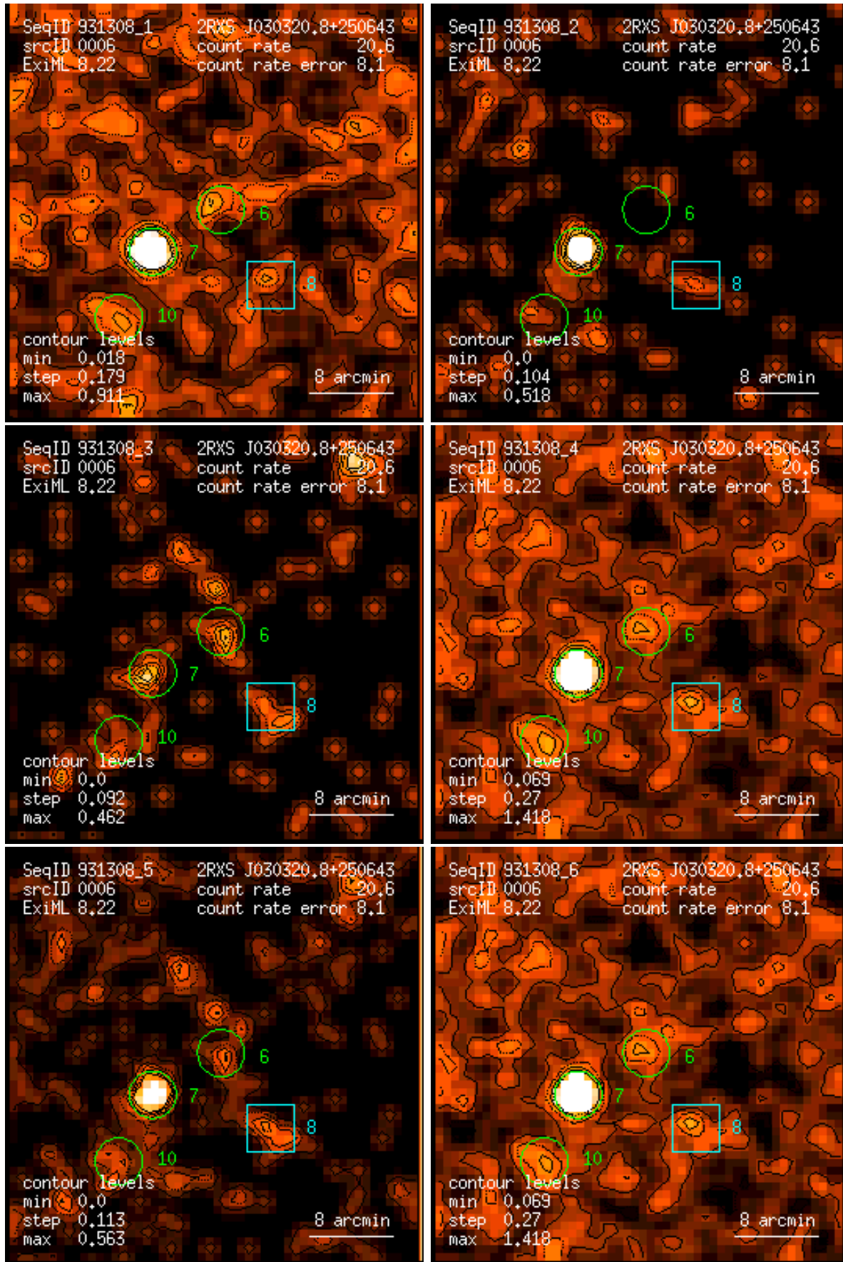
Figure 6: RASS 931308: detection 0006: band rate images, Gaussian filter: (1) PSPC channels 11 – 41, (2) 52 – 90, (3) 91 – 201, (4) 11 – 235, (5) 52 – 201, (6) 11 – 201. Broad band rates in counts/ks. Band rate contour levels in counts/ks/arcmin 2 .
