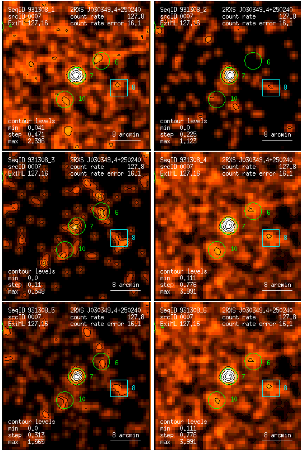
Figure 7: RASS 931308: detection 0007: band rate images, Gaussian filter: (1) PSPC channels 11 – 41, (2) 52 – 90, (3) 91 – 201, (4) 11 – 235, (5) 52 – 201, (6) 11 – 201. Broad band rates in counts/ks. Band rate contour levels in counts/ks/arcmin 2 .
