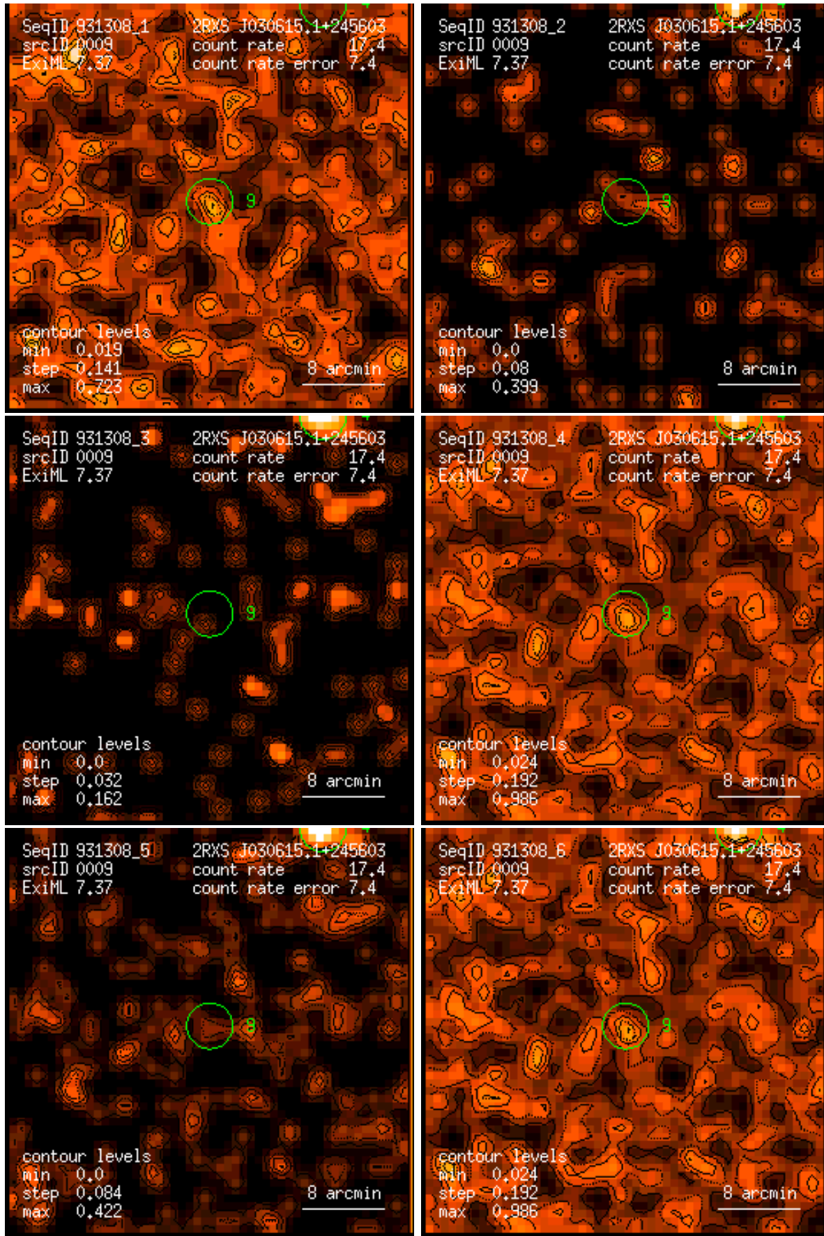
Figure 9: RASS 931308: detection 0009: band rate images, Gaussian filter: (1) PSPC channels 11 – 41, (2) 52 – 90, (3) 91 – 201, (4) 11 – 235, (5) 52 – 201, (6) 11 – 201. Broad band rates in counts/ks. Band rate contour levels in counts/ks/arcmin 2 .
