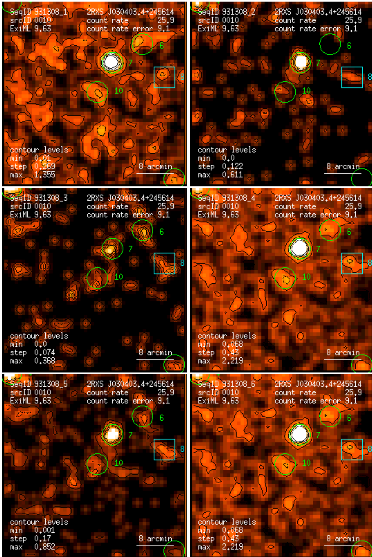
Figure 10: RASS 931308: detection 0010: band rate images, Gaussian filter: (1) PSPC channels 11 – 41, (2) 52 – 90, (3) 91 – 201, (4) 11 – 235, (5) 52 – 201, (6) 11 – 201. Broad band rates in counts/ks. Band rate contour levels in counts/ks/arcmin 2 .
