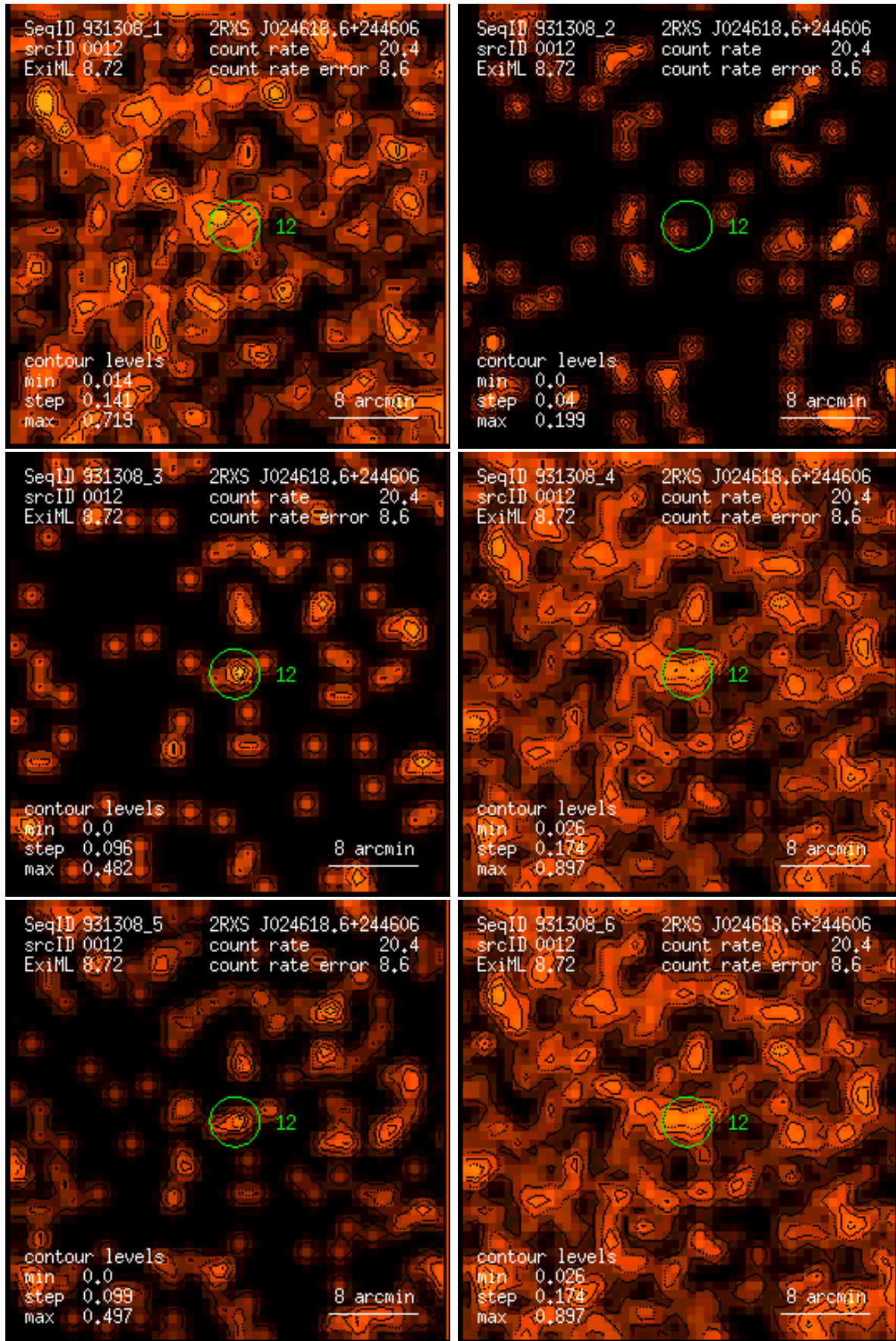
Figure 12: RASS 931308: detection 0012: band rate images, Gaussian filter: (1) PSPC channels 11 – 41, (2) 52 – 90, (3) 91 – 201, (4) 11 – 235, (5) 52 – 201, (6) 11 – 201. Broad band rates in counts/ks. Band rate contour levels in counts/ks/arcmin 2 .
