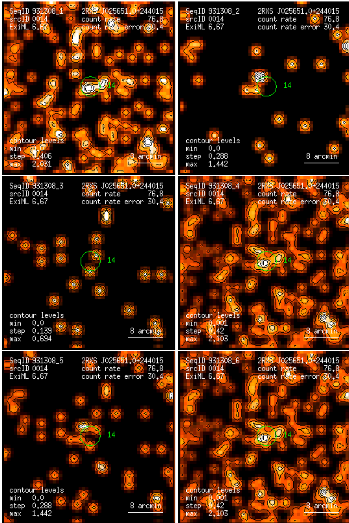
Figure 14: RASS 931308: detection 0014: band rate images, Gaussian filter: (1) PSPC channels 11 – 41, (2) 52 – 90, (3) 91 – 201, (4) 11 – 235, (5) 52 – 201, (6) 11 – 201. Broad band rates in counts/ks. Band rate contour levels in counts/ks/arcmin 2 .
