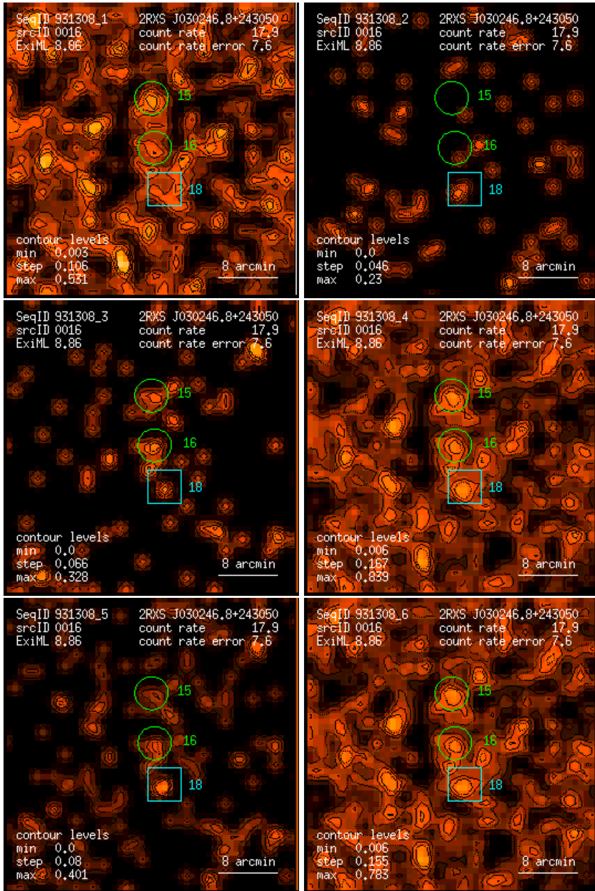
Figure 16: RASS 931308: detection 0016: band rate images, Gaussian filter: (1) PSPC channels 11 – 41, (2) 52 – 90, (3) 91 – 201, (4) 11 – 235, (5) 52 – 201, (6) 11 – 201. Broad band rates in counts/ks. Band rate contour levels in counts/ks/arcmin 2 .
