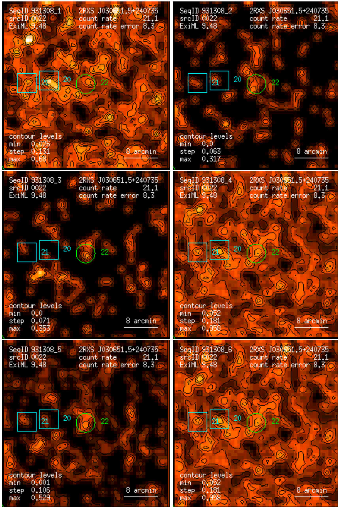
Figure 22: RASS 931308: detection 0022: band rate images, Gaussian filter: (1) PSPC channels 11 – 41, (2) 52 – 90, (3) 91 – 201, (4) 11 – 235, (5) 52 – 201, (6) 11 – 201. Broad band rates in counts/ks. Band rate contour levels in counts/ks/arcmin 2 .
