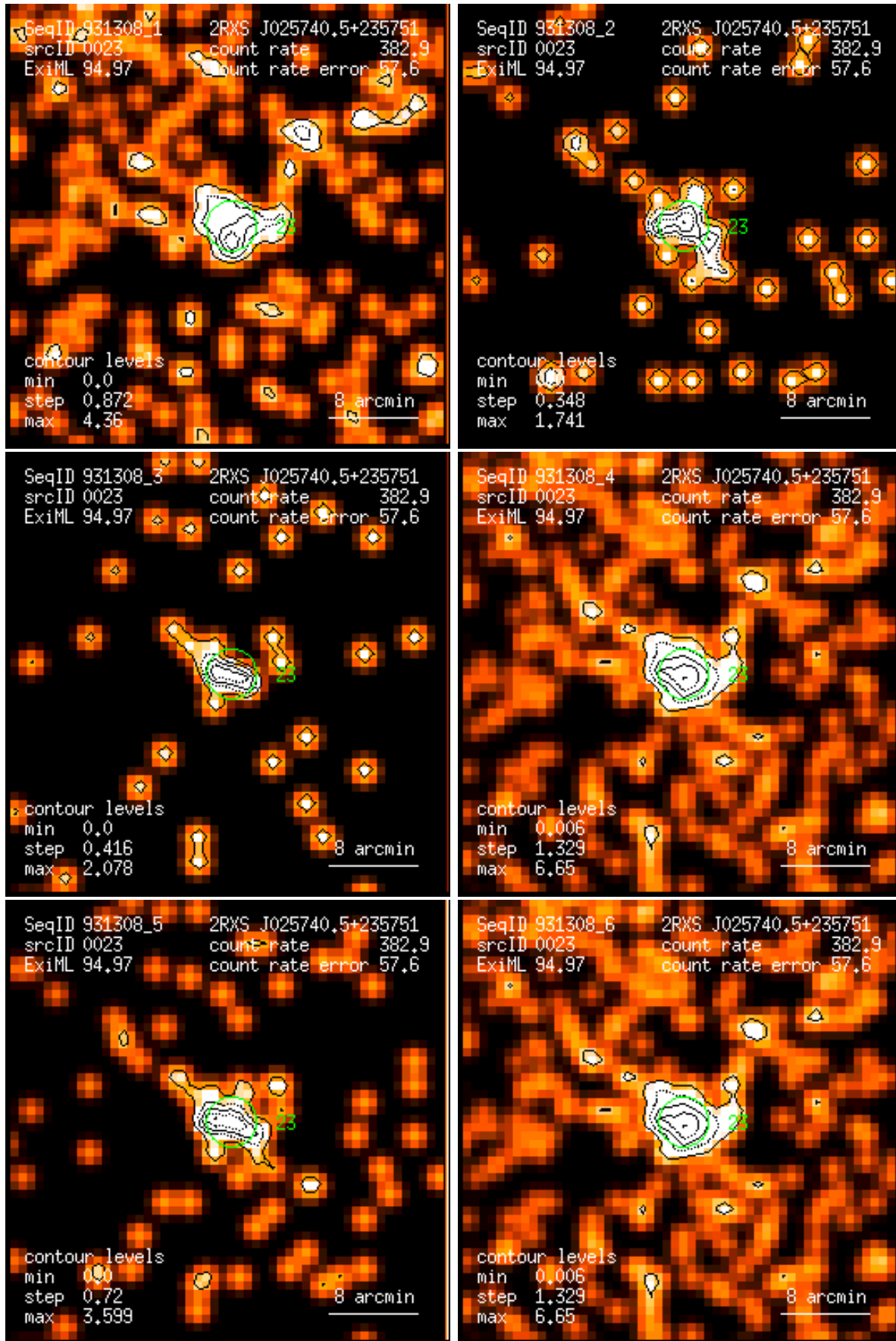
Figure 23: RASS 931308: detection 0023: band rate images, Gaussian filter: (1) PSPC channels 11 – 41, (2) 52 – 90, (3) 91 – 201, (4) 11 – 235, (5) 52 – 201, (6) 11 – 201. Broad band rates in counts/ks. Band rate contour levels in counts/ks/arcmin 2 .
