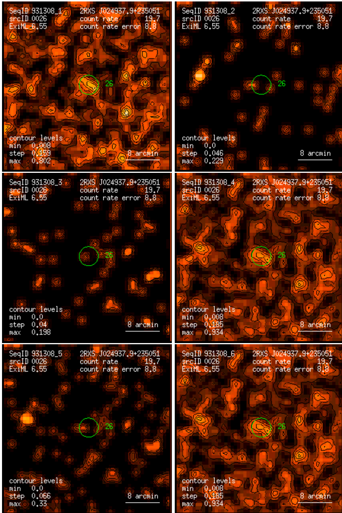
Figure 26: RASS 931308: detection 0026: band rate images, Gaussian filter: (1) PSPC channels 11 – 41, (2) 52 – 90, (3) 91 – 201, (4) 11 – 235, (5) 52 – 201, (6) 11 – 201. Broad band rates in counts/ks. Band rate contour levels in counts/ks/arcmin 2 .
