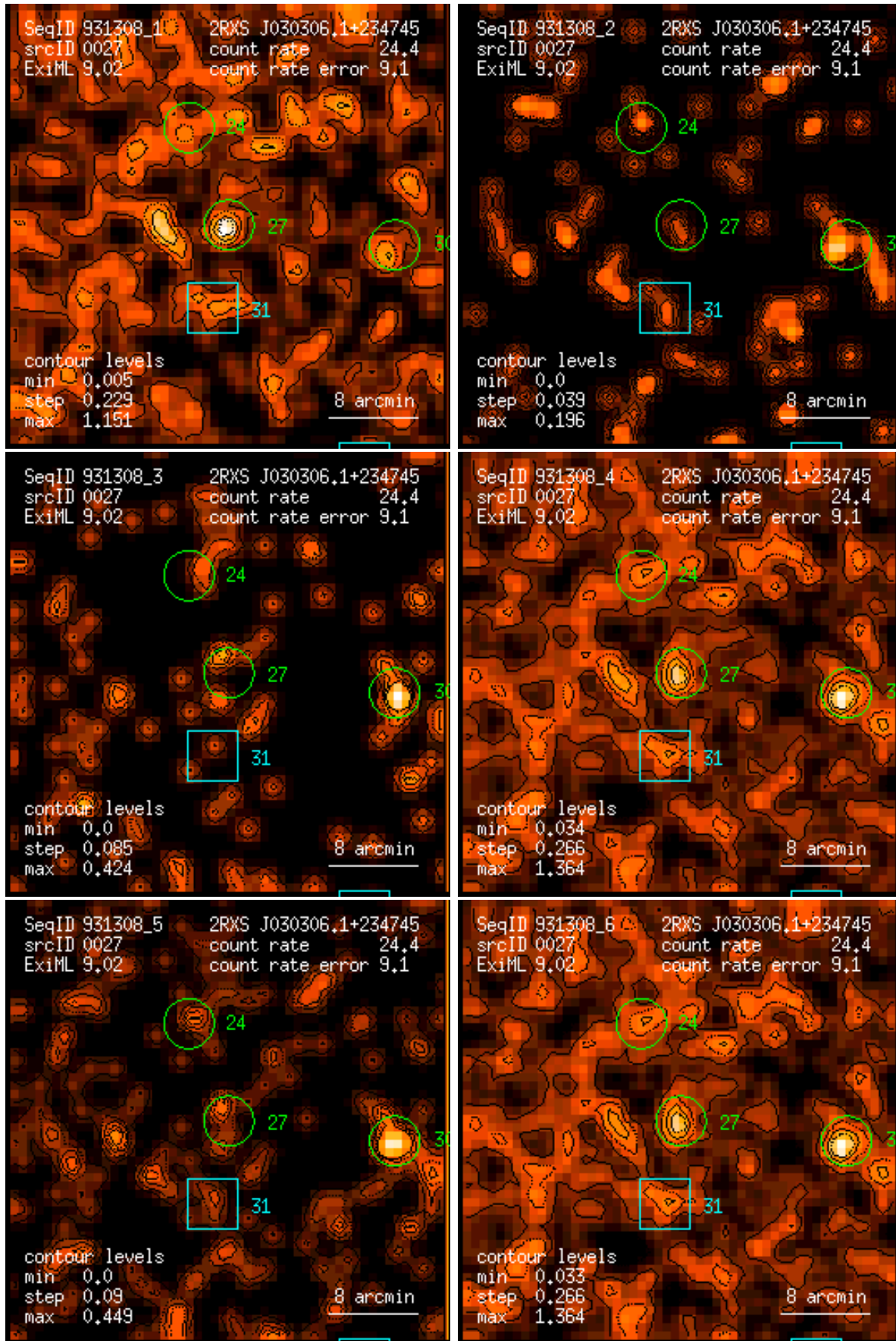
Figure 27: RASS 931308: detection 0027: band rate images, Gaussian filter: (1) PSPC channels 11 – 41, (2) 52 – 90, (3) 91 – 201, (4) 11 – 235, (5) 52 – 201, (6) 11 – 201. Broad band rates in counts/ks. Band rate contour levels in counts/ks/arcmin 2 .
