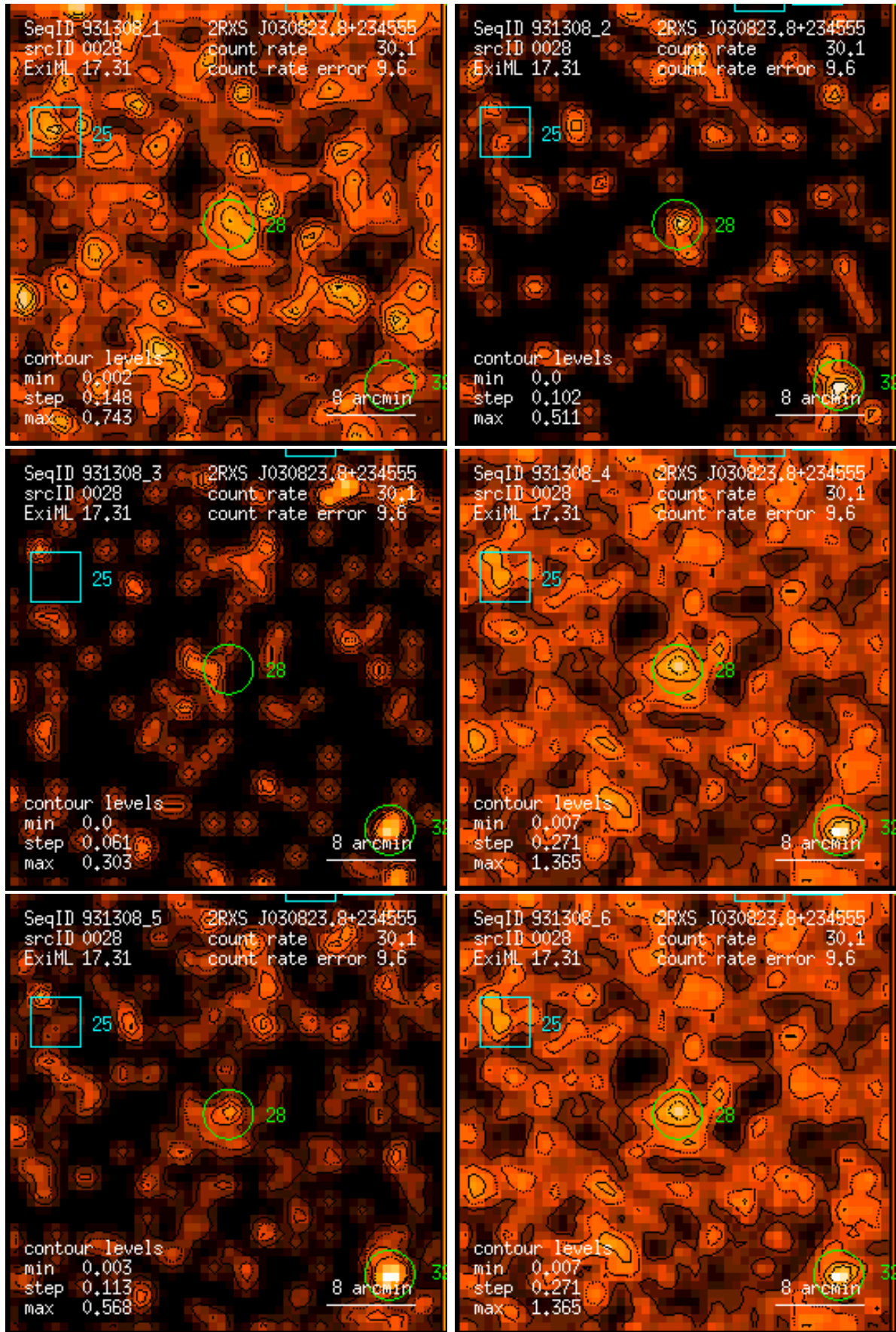
Figure 28: RASS 931308: detection 0028: band rate images, Gaussian filter: (1) PSPC channels 11 – 41, (2) 52 – 90, (3) 91 – 201, (4) 11 – 235, (5) 52 – 201, (6) 11 – 201. Broad band rates in counts/ks. Band rate contour levels in counts/ks/arcmin 2 .
