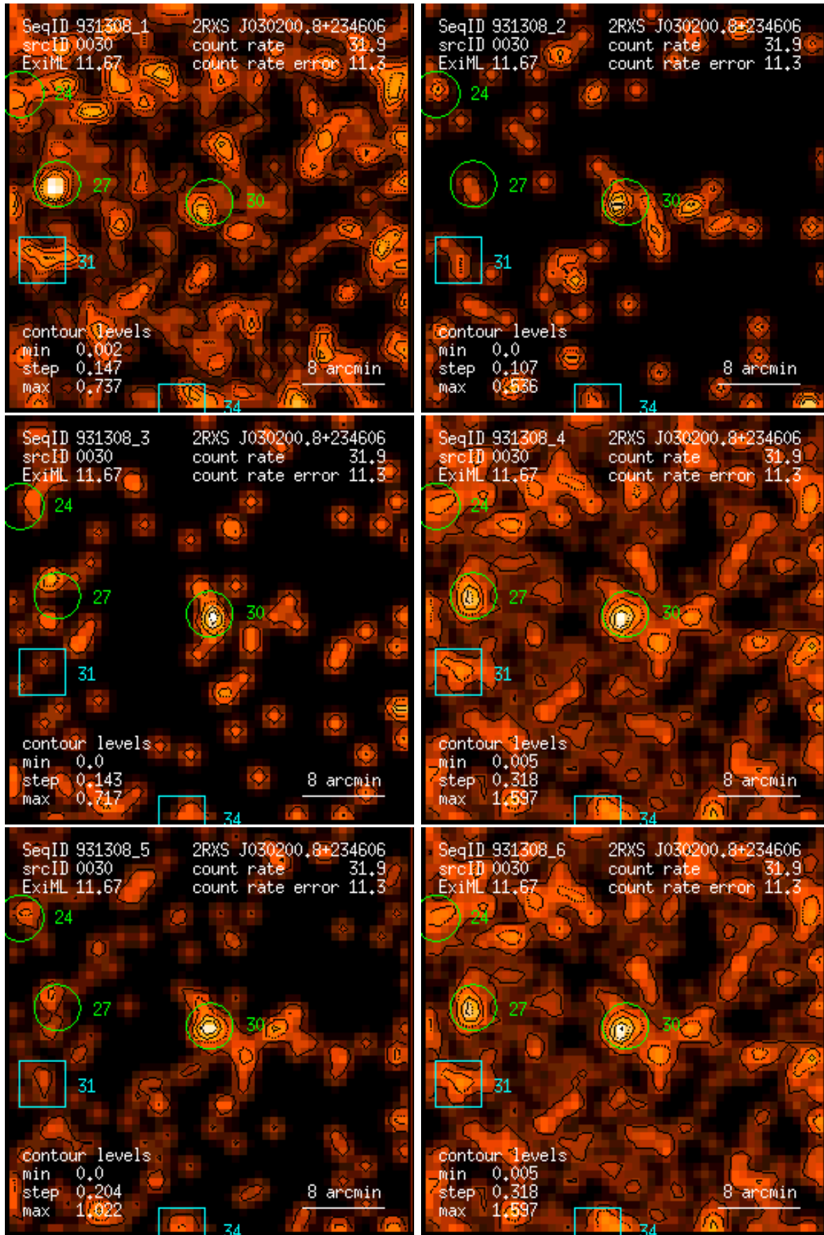
Figure 30: RASS 931308: detection 0030: band rate images, Gaussian filter: (1) PSPC channels 11 – 41, (2) 52 – 90, (3) 91 – 201, (4) 11 – 235, (5) 52 – 201, (6) 11 – 201. Broad band rates in counts/ks. Band rate contour levels in counts/ks/arcmin 2 .
