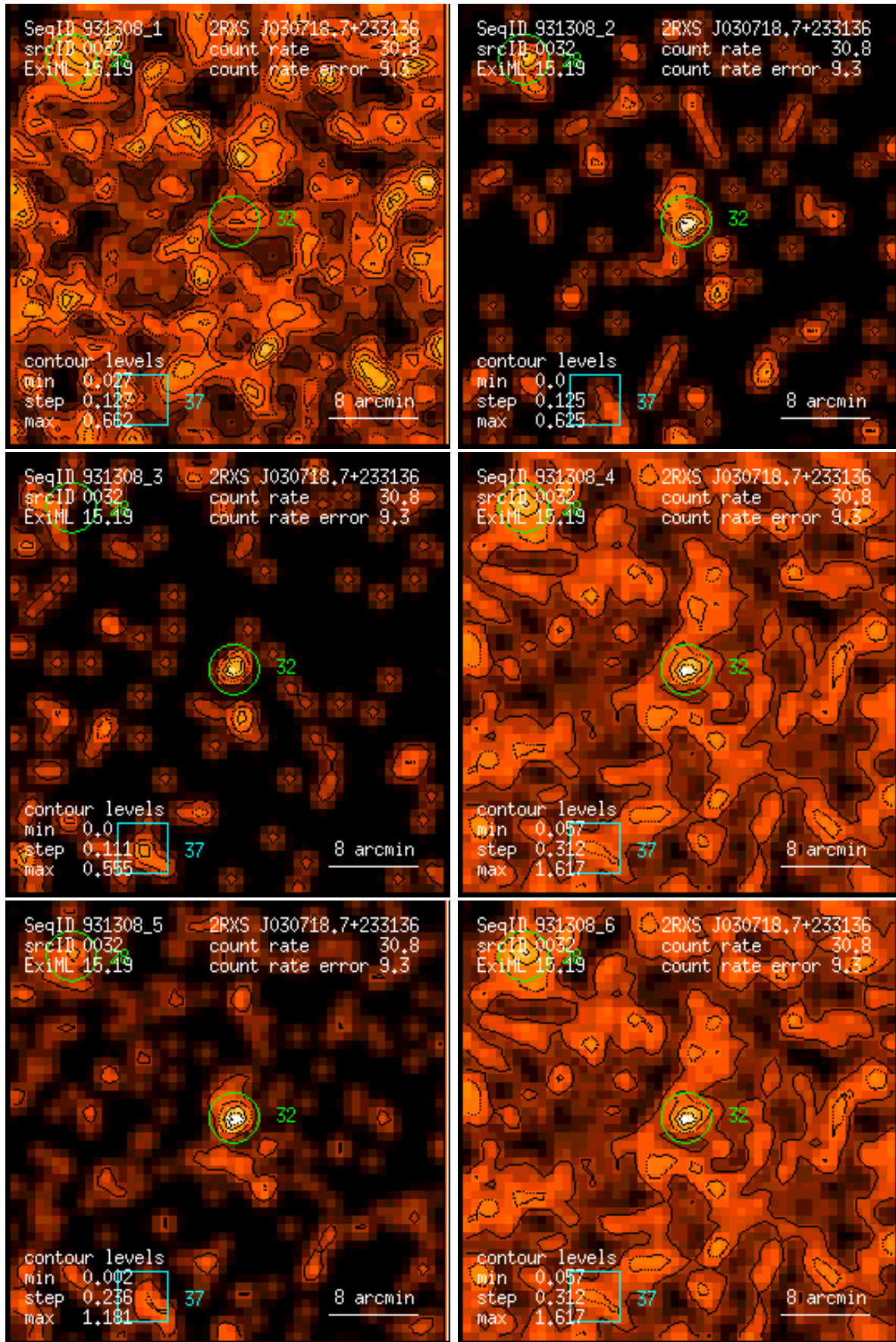
Figure 32: RASS 931308: detection 0032: band rate images, Gaussian filter: (1) PSPC channels 11 – 41, (2) 52 – 90, (3) 91 – 201, (4) 11 – 235, (5) 52 – 201, (6) 11 – 201. Broad band rates in counts/ks. Band rate contour levels in counts/ks/arcmin 2 .
