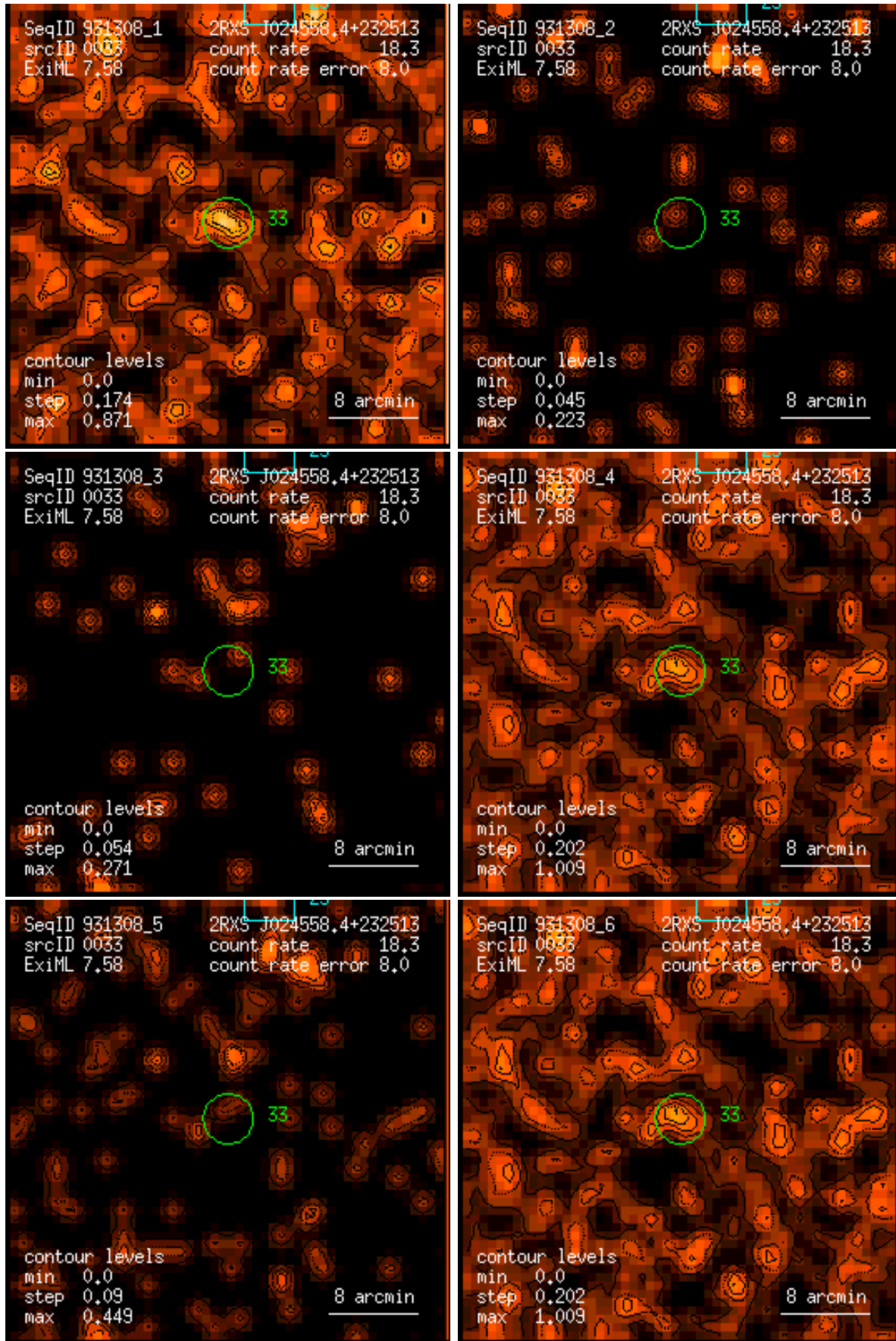
Figure 33: RASS 931308: detection 0033: band rate images, Gaussian filter: (1) PSPC channels 11 – 41, (2) 52 – 90, (3) 91 – 201, (4) 11 – 235, (5) 52 – 201, (6) 11 – 201. Broad band rates in counts/ks. Band rate contour levels in counts/ks/arcmin 2 .
