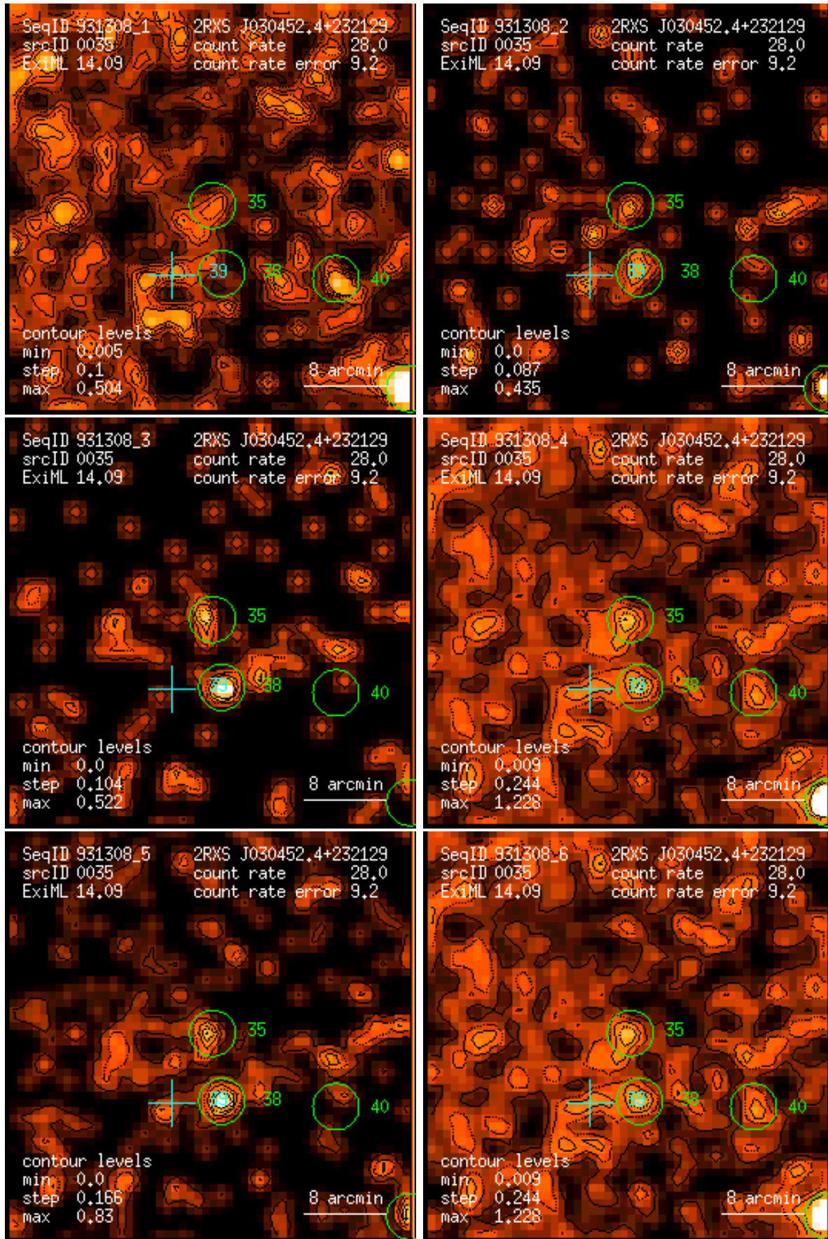
Figure 35: RASS 931308: detection 0035: band rate images, Gaussian filter: (1) PSPC channels 11 – 41, (2) 52 – 90, (3) 91 – 201, (4) 11 – 235, (5) 52 – 201, (6) 11 – 201. Broad band rates in counts/ks. Band rate contour levels in counts/ks/arcmin 2 .
