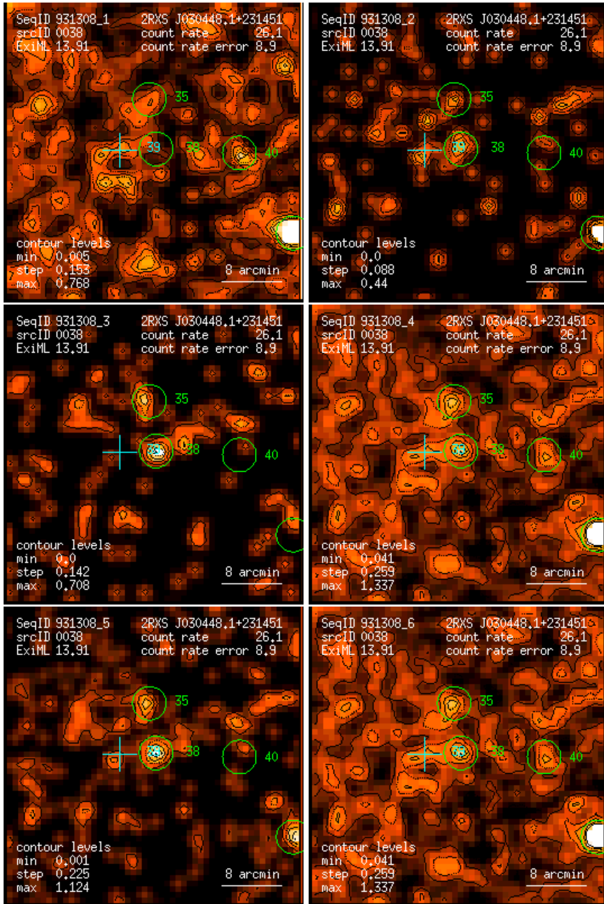
Figure 38: RASS 931308: detection 0038: band rate images, Gaussian filter: (1) PSPC channels 11 – 41, (2) 52 – 90, (3) 91 – 201, (4) 11 – 235, (5) 52 – 201, (6) 11 – 201. Broad band rates in counts/ks. Band rate contour levels in counts/ks/arcmin 2 .
