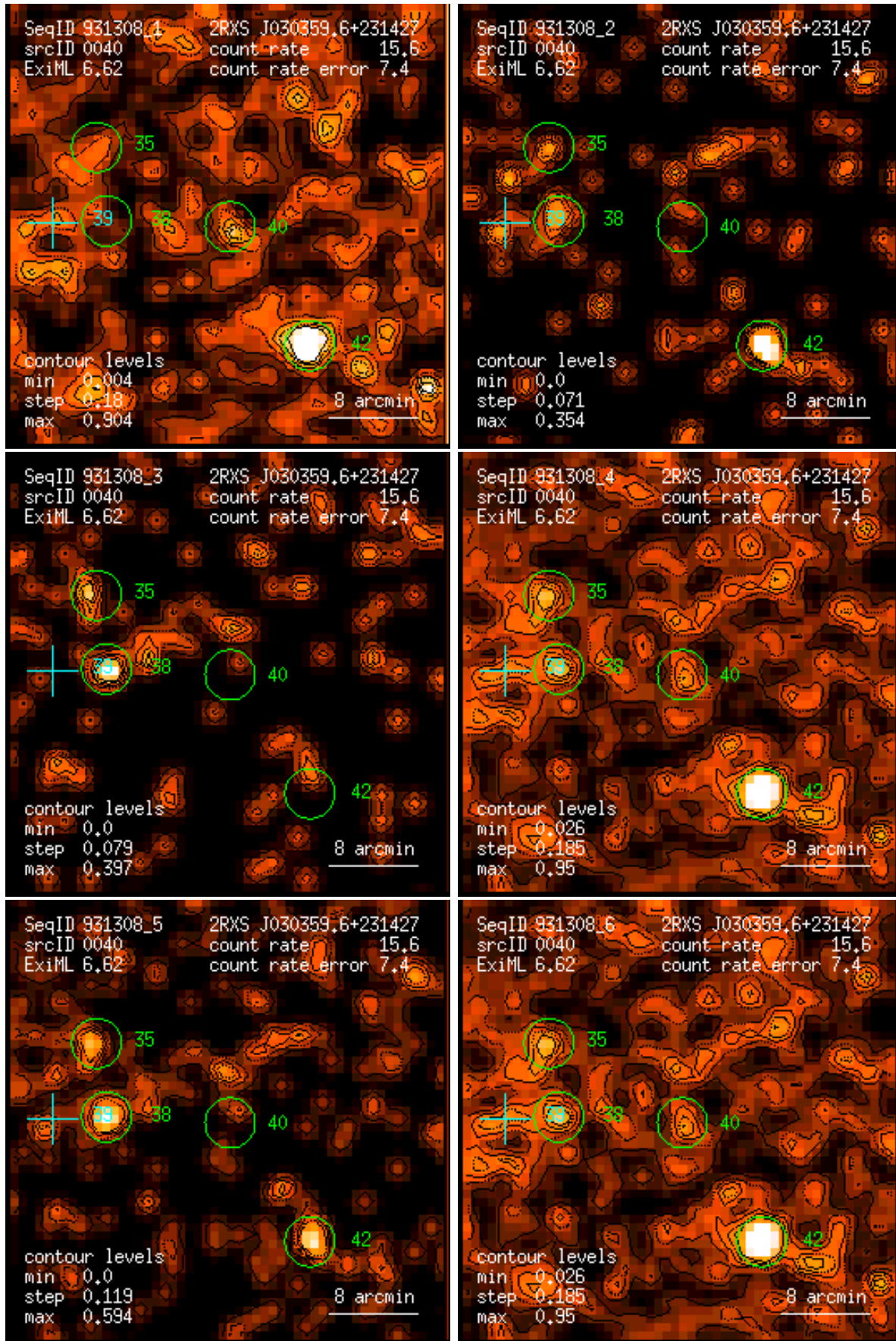
Figure 40: RASS 931308: detection 0040: band rate images, Gaussian filter: (1) PSPC channels 11 – 41, (2) 52 – 90, (3) 91 – 201, (4) 11 – 235, (5) 52 – 201, (6) 11 – 201. Broad band rates in counts/ks. Band rate contour levels in counts/ks/arcmin 2 .
