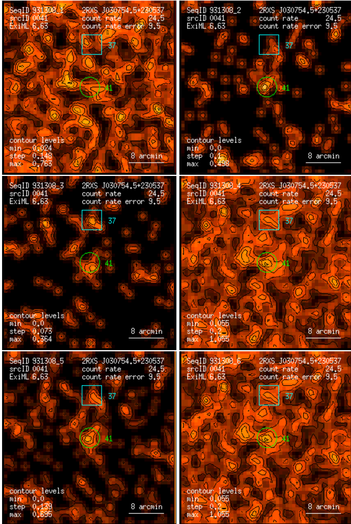
Figure 41: RASS 931308: detection 0041: band rate images, Gaussian filter: (1) PSPC channels 11 – 41, (2) 52 – 90, (3) 91 – 201, (4) 11 – 235, (5) 52 – 201, (6) 11 – 201. Broad band rates in counts/ks. Band rate contour levels in counts/ks/arcmin 2 .
