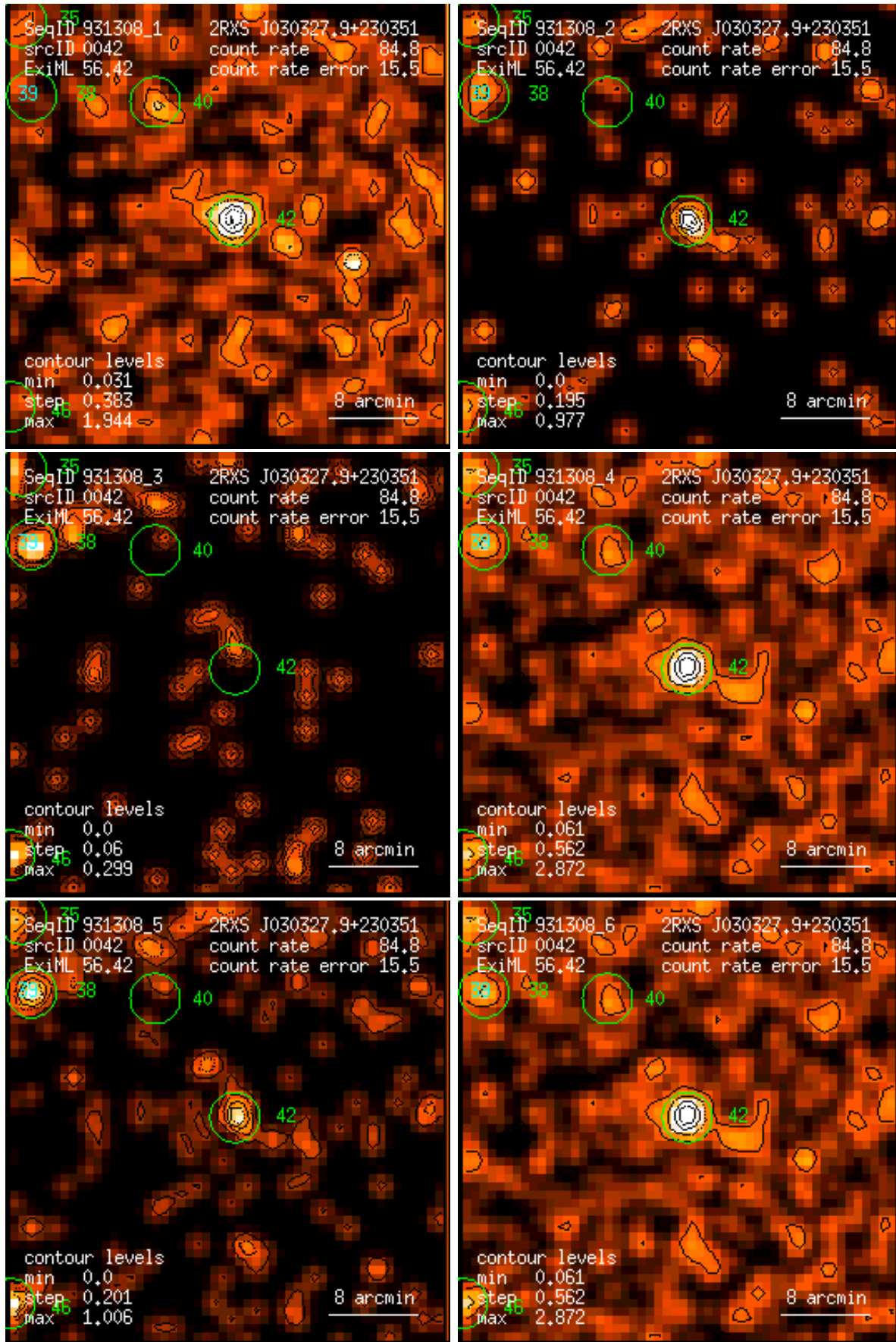
Figure 42: RASS 931308: detection 0042: band rate images, Gaussian filter: (1) PSPC channels 11 – 41, (2) 52 – 90, (3) 91 – 201, (4) 11 – 235, (5) 52 – 201, (6) 11 – 201. Broad band rates in counts/ks. Band rate contour levels in counts/ks/arcmin 2 .
