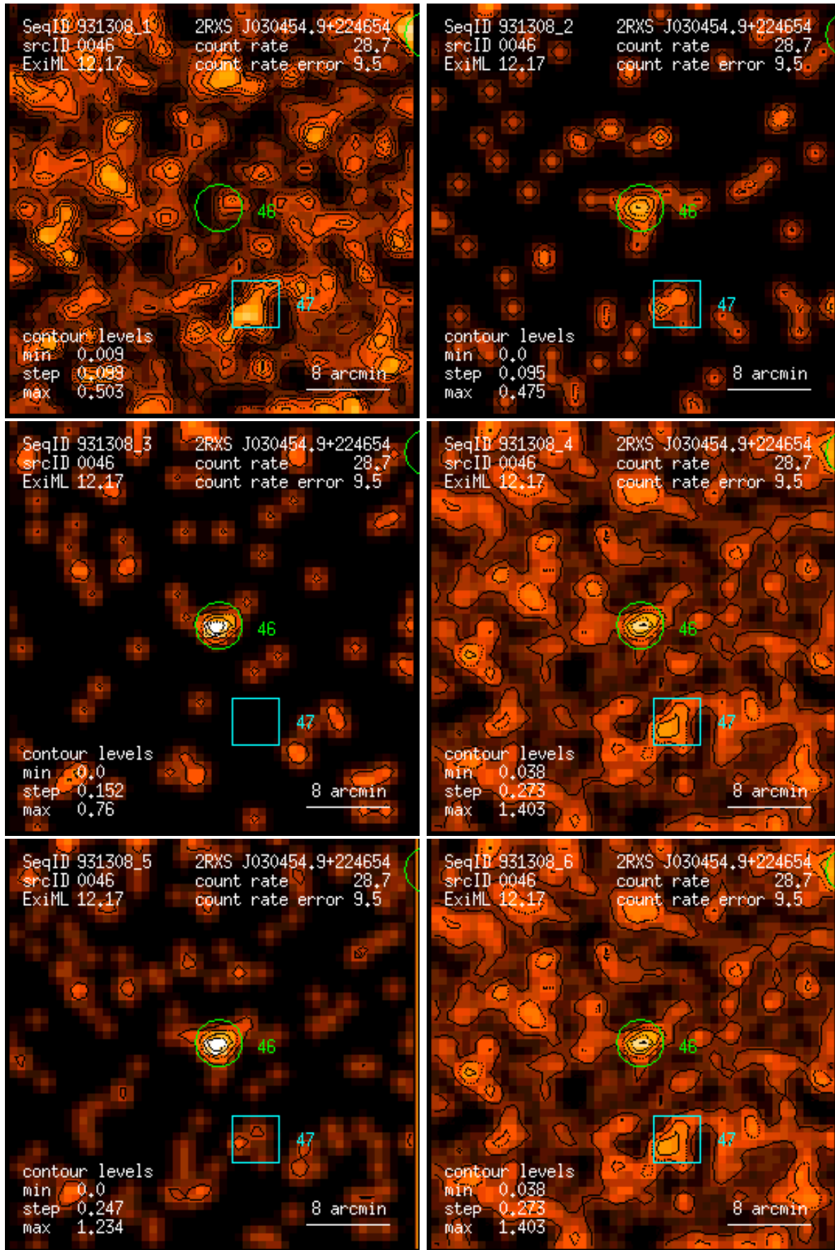
Figure 46: RASS 931308: detection 0046: band rate images, Gaussian filter: (1) PSPC channels 11 – 41, (2) 52 – 90, (3) 91 – 201, (4) 11 – 235, (5) 52 – 201, (6) 11 – 201. Broad band rates in counts/ks. Band rate contour levels in counts/ks/arcmin 2 .
