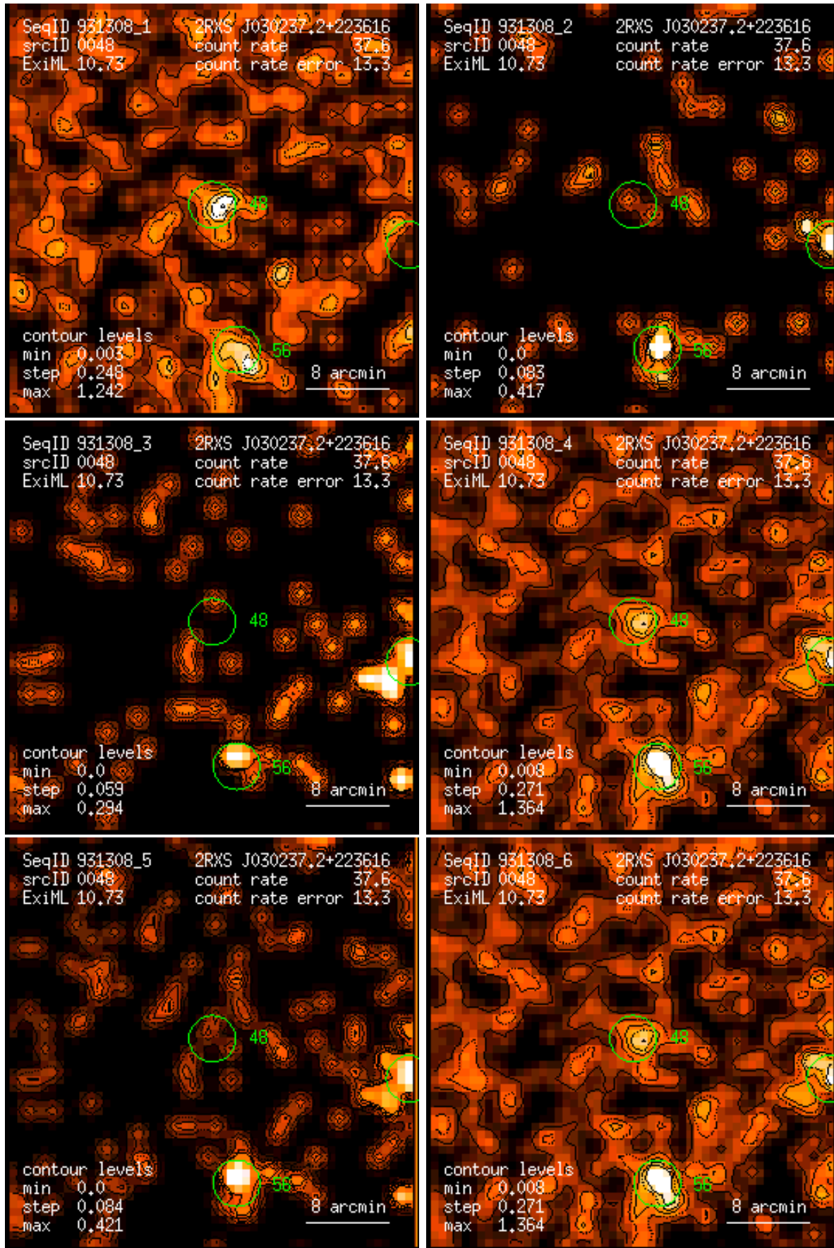
Figure 48: RASS 931308: detection 0048: band rate images, Gaussian filter: (1) PSPC channels 11 – 41, (2) 52 – 90, (3) 91 – 201, (4) 11 – 235, (5) 52 – 201, (6) 11 – 201. Broad band rates in counts/ks. Band rate contour levels in counts/ks/arcmin 2 .
