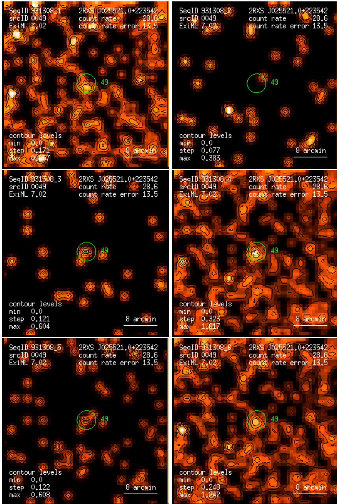
Figure 49: RASS 931308: detection 0049: band rate images, Gaussian filter: (1) PSPPC channels 11 – 41, (2) 52 – 90, (3) 91 – 201, (4) 11 – 235, (5) 52 – 201, (6) 11 – 201. Broad band rates in counts/ks. Band rate contour levels in counts/ks/arcmin 2 .
