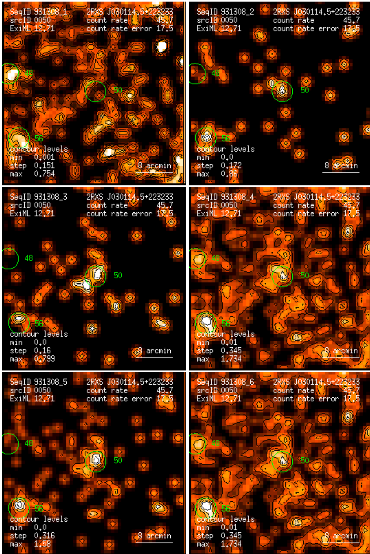
Figure 50: RASS 931308: detection 0050: band rate images, Gaussian filter: (1) PSPC channels 11 – 41, (2) 52 – 90, (3) 91 – 201, (4) 11 – 235, (5) 52 – 201, (6) 11 – 201. Broad band rates in counts/ks. Band rate contour levels in counts/ks/arcmin 2 .
