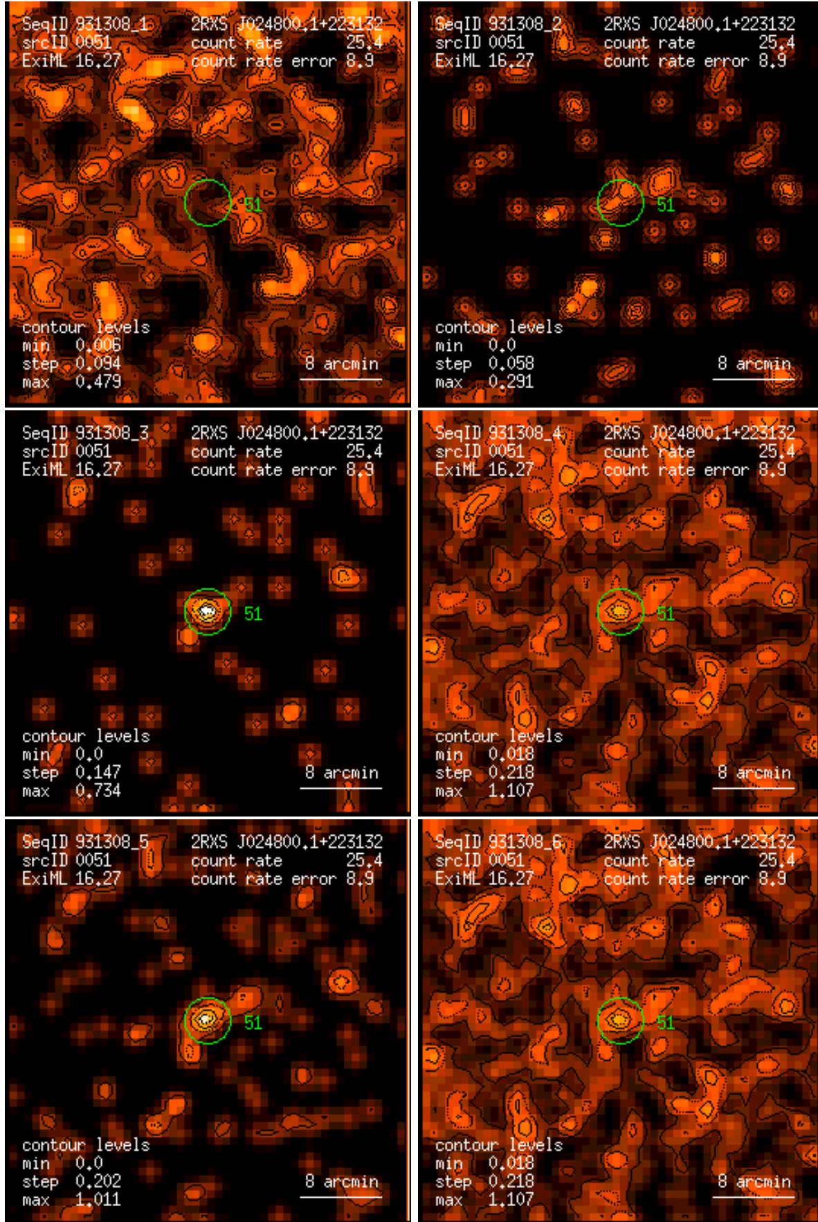
Figure 51: RASS 931308: detection 0051: band rate images, Gaussian filter: (1) PSPC channels 11 – 41, (2) 52 – 90, (3) 91 – 201, (4) 11 – 235, (5) 52 – 201, (6) 11 – 201. Broad band rates in counts/ks. Band rate contour levels in counts/ks/arcmin 2 .
